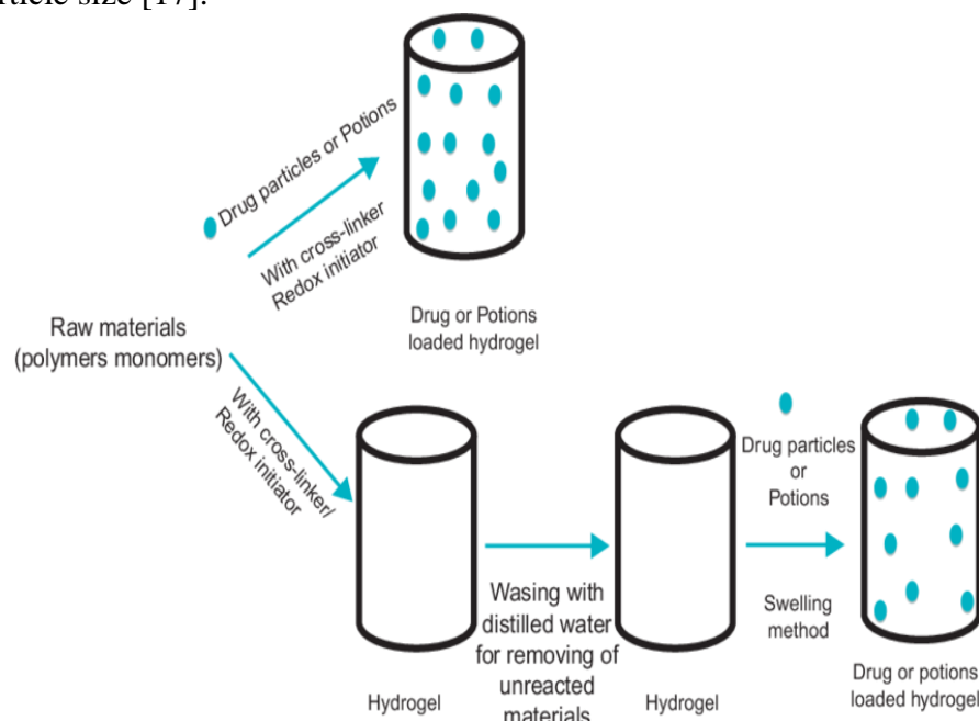
Figure 7: Polymerization Method
