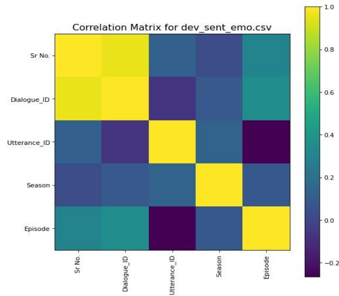
Figure 2: Correlation Matrix
