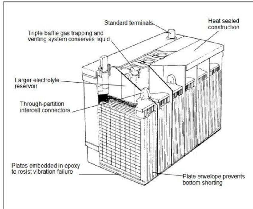
Figure 3: Lead-Acid Battery
