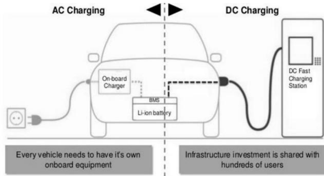
Figure1: Charging Station for EV
