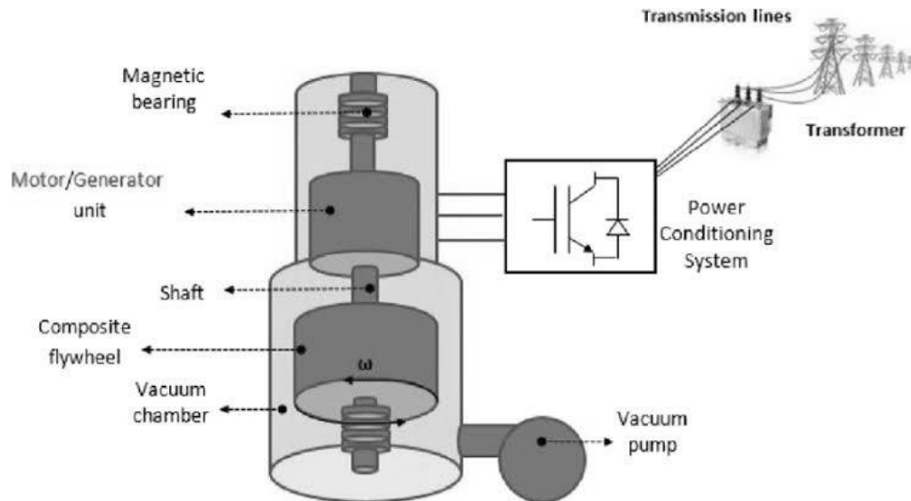
Figure 2: Flywheel Storage System
