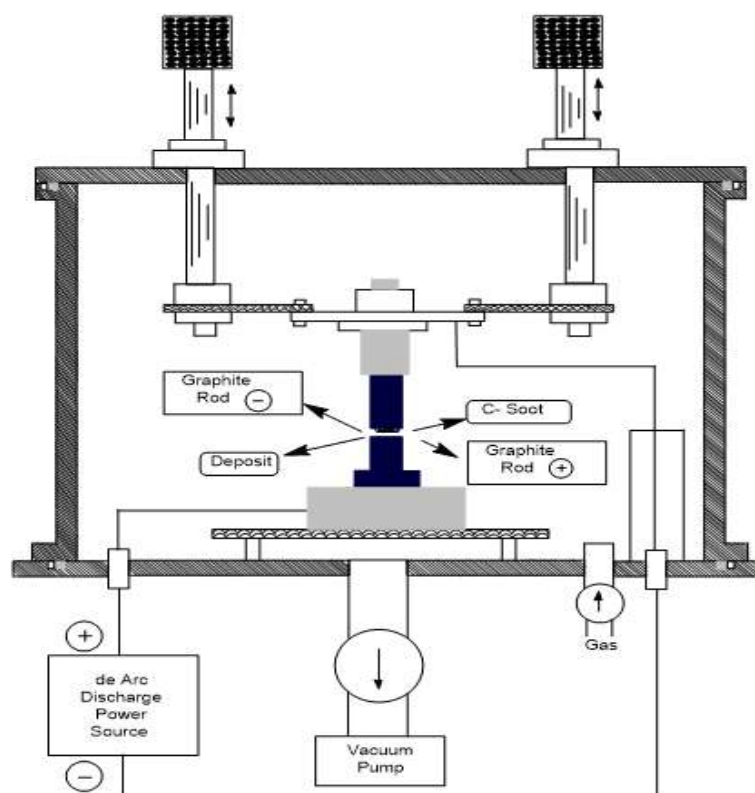
Figure 1: Arc evaporation apparatus for producing CNTs
