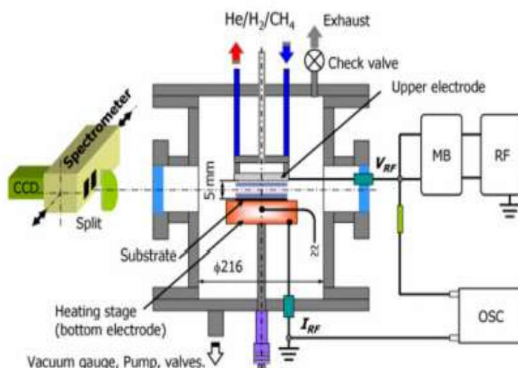
Figure 3: Measurement system and reactor of APRFD. Reprinted with permission from Nozaki, T., Ohnishi, K., Okazaki, K. & Kortshagen, U. Fabrication of vertically aligned single-walled carbon nanotubes in atmospheric pressure non-thermal plasma CVD. Carbon N. Y. 45, 364–374 (2007). Copyright (2007) Elsevier Ltd.
