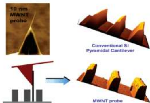
Figure 7: Comparison of the AFM depictions captured from the multiwalled CNT probe and the silicon probe. (Valcárcel et al., 2007) Reprinted with permission from Valcárcel, M., Cárdenas, S. & Simonet, B. M. Role of Carbon Nanotubes in Analytical Science. Anal. Chem. 79, 4788–4797 (2007). Copyright (2007) American Chemical Society.
