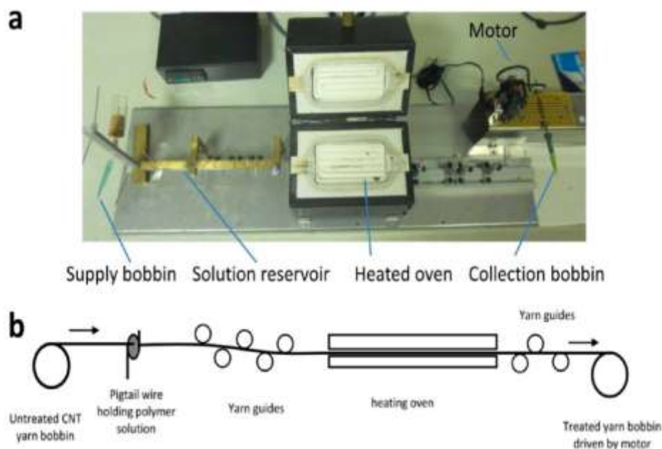
Figure 12: (a) Image, and (b) graphic of the continual dip-coating line utilized for the solution polyaniline nanowire and the gel PVA-H 3 PO 4 . (Su et al., 2014) Reprinted with permission from Su, F., Miao, M., Niu, H. & Wei, Z. Gamma-Irradiated Carbon Nanotube Yarn As Substrate for High-Performance Fiber Supercapacitors. ACS Appl. Mater. Interfaces 6, 2553–2560 (2014). Copyright (2014) American Chemical Society.
