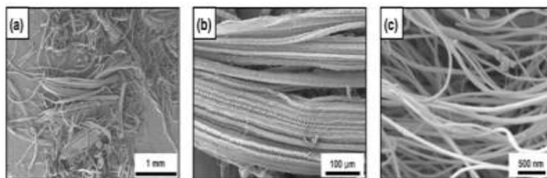
Figure 6: SEM image of the CNTs produced via direct bubbling of C 2 H 2 (flow rate- 30 sccm). (a) SEM micrograph of CNTs (length is nearly 2000 μm). (b) Magnified micrograph of (a). (c) Magnified micrograph of (b) exhibiting average diameter (80-90 nm). Reprinted with permission from Lee, C. J., Lyu, S. C., Kim, H.-W., Park, C.-Y. & Yang, C.-W. Large-scale production of aligned carbon nanotubes by the vapor phase growth method. Chem. Phys. Lett. 359, 109–114 (2002). Copyright (2002) Elsevier Science B.V.
