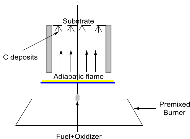
Figure 4: Schematic representation of hydrocarbon flames method for synthesis of CNTs
