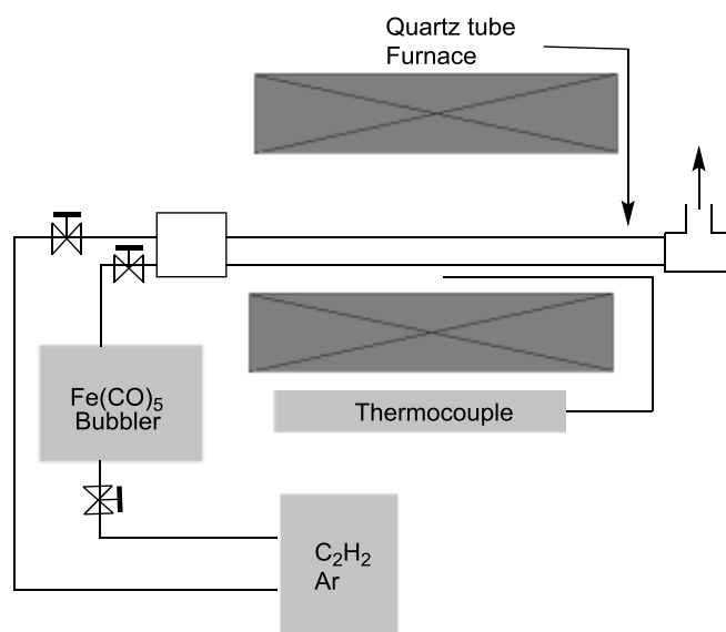
Figure 5: Schematic diagram for the vapor phase growth system.
