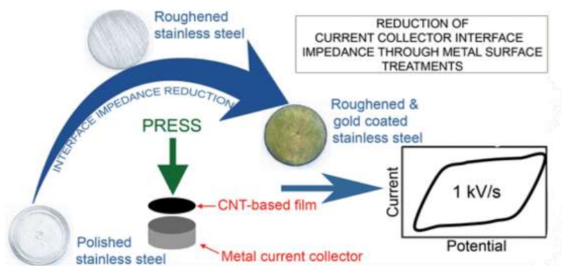
Figure- 13 : Metal surface treatment for interface impedance reduction.(Rangom et al., 2015)Reprinted with permission from Rangom, Y., Tang, X. (Shirley) & Nazar, L. F. Carbon Nanotube-Based Supercapacitors with Excellent ac Line Filtering and Rate Capability via Improved Interfacial Impedance. ACS Nano 9, 7248–7255 (2015) Copyright (2015) American Chemical Society.
