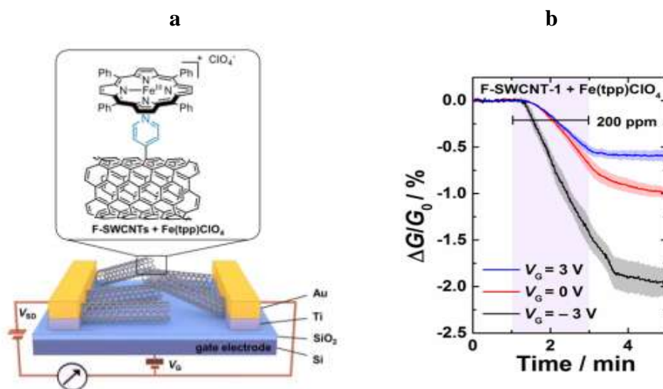
Figure 8: (a) Schematic illustration of the CO sensor encompassing iron porphyrin and SWCNTs (pyridyl-functionalized). (b) The Conductance curves of the sensor F-SWCNT-1 along with \text{Fe}(\text{tpp})\text{ClO}_4 towards exposure of 2 min at 200 ppm of CO at a gate voltage of +3, 0, -3 V. (Savagatrup et al., 2017) Reprinted with permission from Savagatrup, S. et al. Bio-Inspired Carbon Monoxide Sensors with Voltage-Activated Sensitivity. Angew. Chemie 129, 14254–14258 (2017). Copyright (2017) Wiley-VCH Verlag GmbH & Co. KGaA, Weinheim.
