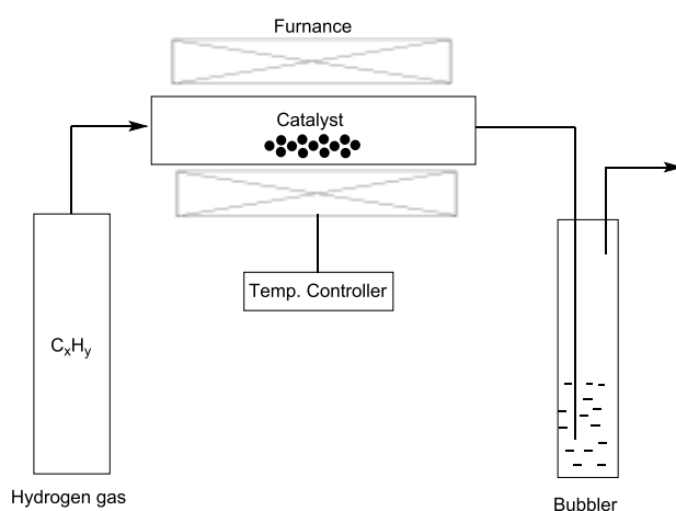
Figure 2: The Schematic diagram of the CVD experimental setup
