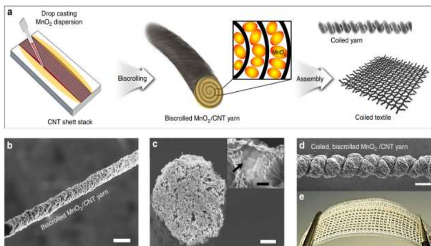
Figure 11: Schematic illustration of (a) Schematic description of MnO_2 -loaded bisrolled yarn electrode and bisrolled yarn-based coiled supercapacitor fabrication. (b,c) SEM morphology of bisrolled MnO_2 /CNT yarn electrode and its cross-section (d) SEM image of the 5-ply, bisrolled MnO_2 /CNT yarn coiled via twist insertion (e) Photograph of non-coiled bisrolled yarn electrodes knitted into a fabric.(Choi et al., 2016) (a) Reprinted with permission from Choi, C. et al. Improvement of system capacitance via weavable superelastic bisrolled yarn supercapacitors. Nat. Commun. 7, 13811 (2016). Copyright (2016) Springer Nature.
