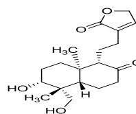
14-deoxyandrographolide (4)
