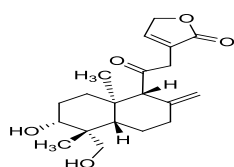
14-deoxy-11-oxoandrographolide (5)
