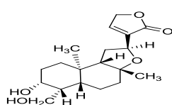
Isoandrographolide (3)
