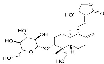
3-O- \beta -D-glucopyranoylandrographolide (9)
