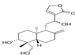
14-deoxy-12-dehydroxy- andrographolide (7)
