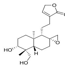
8,17-Epoxy-14-deoxyandrographolide (10)
