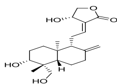
Andrographolide (1)
