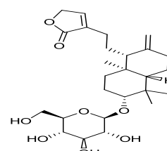
3-O-β-D-glucopyranosyl-14,19- dideoxyandrographolide (8)
