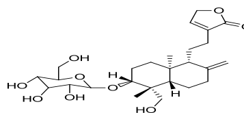
3-O-β-D-glucosyl-deoxyandrographolide (6)
