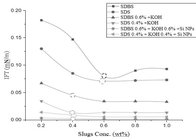
Graph 1: IFT (mN/m) v/s concentration of various slugs (wt%) and determining CMC.
