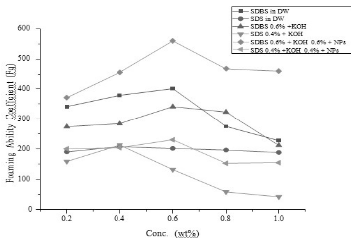
Graph 2: Effect of surfactant type and concentration on foaming ability coefficient in DW along with KOH and Silica NPs
