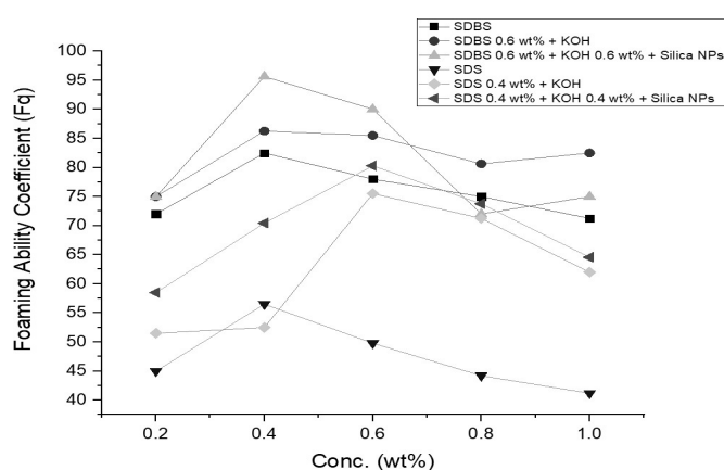
Graph 3: Effect of surfactant type and concentration on foaming ability coefficient in crude oil along with KOH and Silica NPs
