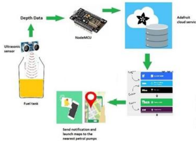
Figure 1: Components of Proposed System
