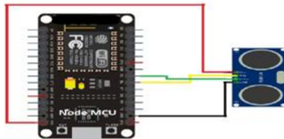
Figure 2: Schematic of NodeMCU with ultrasonic sensor
