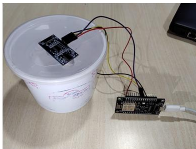
Figure 5: Fuel Level Monitoring System
