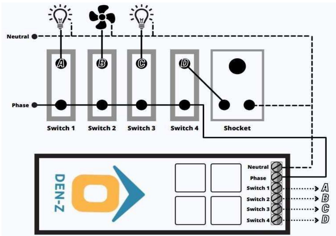
Figure 8: Connection Diagram
