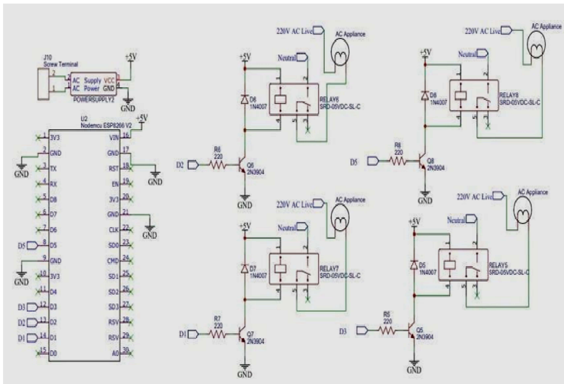
Figure 7: Circuit Diagram
