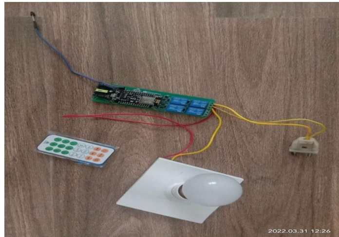
Figure 9: Working Model
