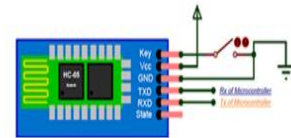
Figure 4: Bluetooth Module HC-05
