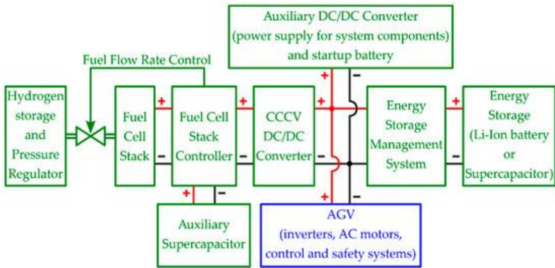
Figure 7: Energy Storage System for Electric Vehicles
