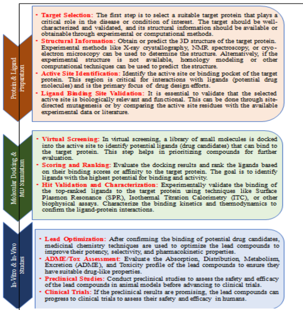
Figure 2: Overview of protein selection and validation
