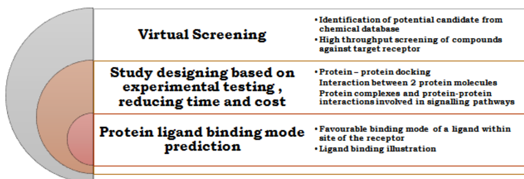
Figure 5: Types of Molecular Docking Techniques
