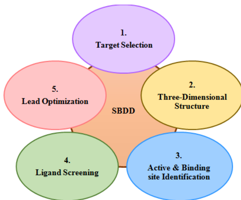
Figure 1: Structure Based Drug Designing Flowchart
