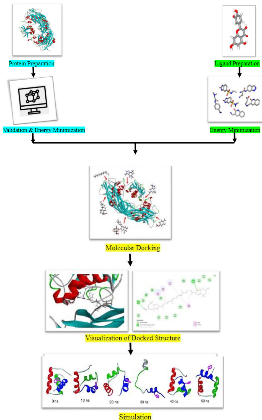
Figure 3: Steps to perform Molecular Docking
