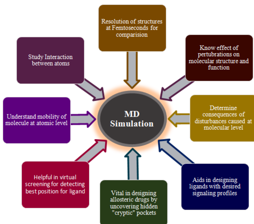
Figure 4: Why should we use MD Simulations
