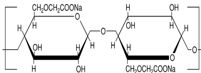
Figure 5: Carboxy methyl cellulose sodium
