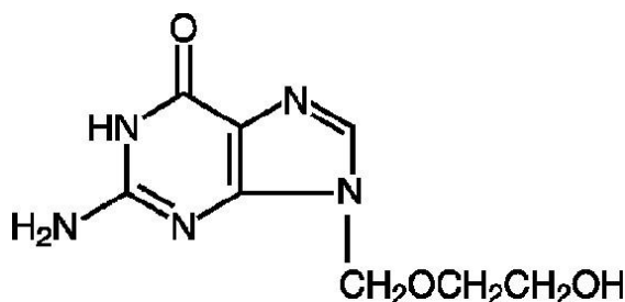
Figure 2: 2-amino-1,9-dihydro-9-[(2-hydroxyethoxy) methyl]-6H-purin-6-one
