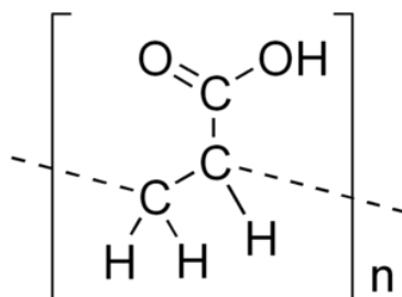
Figure 3: Poly (acrylic acid), poly(1-carboxyethylene)
