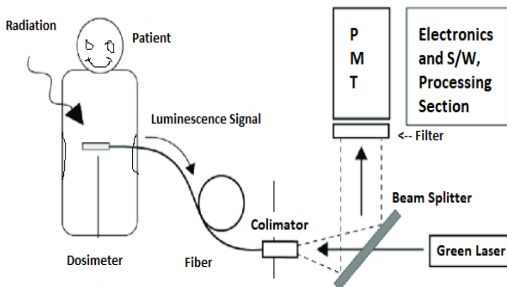
Figure 3: Basic concept of radioluminescence dosimetry.
