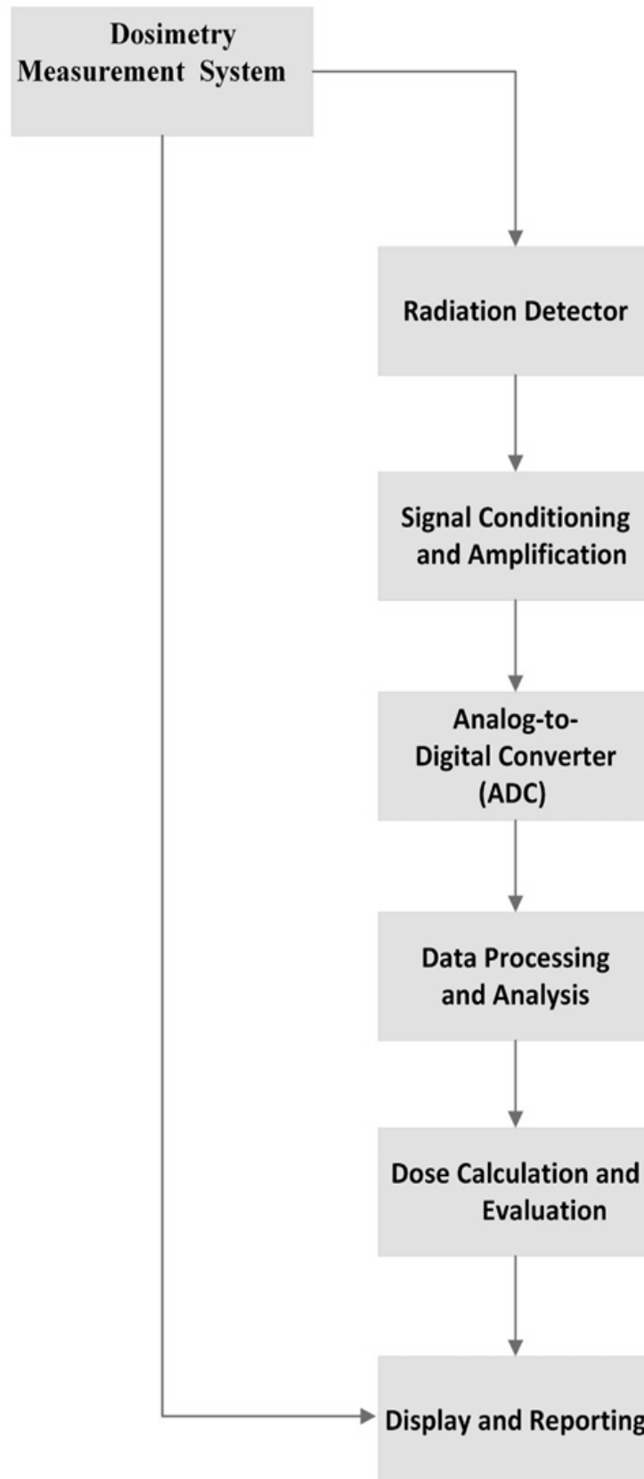
Figure 2: Block Diagram representing a generic Dosimetry measurement system.
