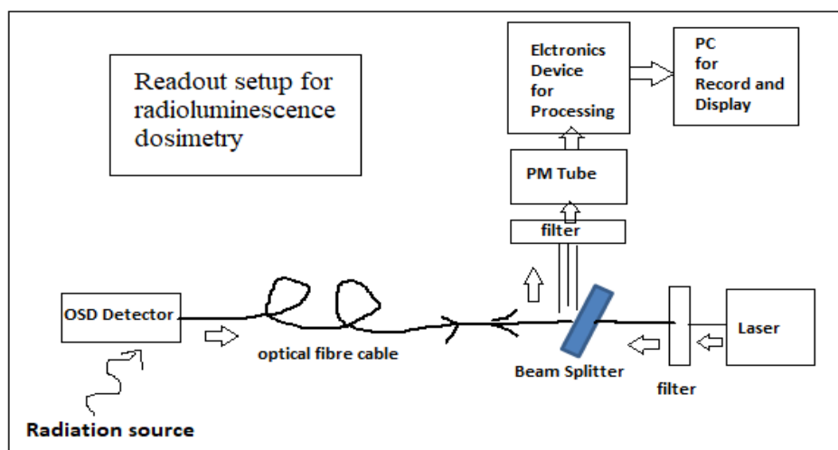
Figure 5: Readout setup for radioluminescence dosimetry.
