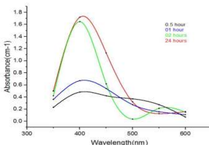
Figure 7: The impact of time on synthesis of silver nanoparticles
