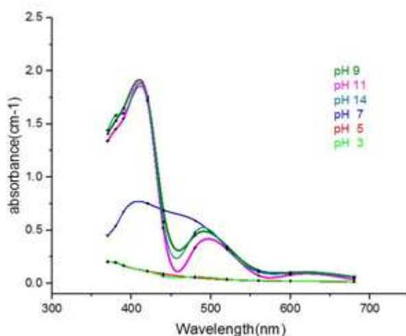
Figure 6: The impact of p H on synthesis of silver Nanoparticles
