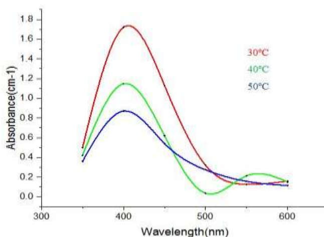
Figure 8: The impact of temperature on the synthesis of silver nanoparticles.
