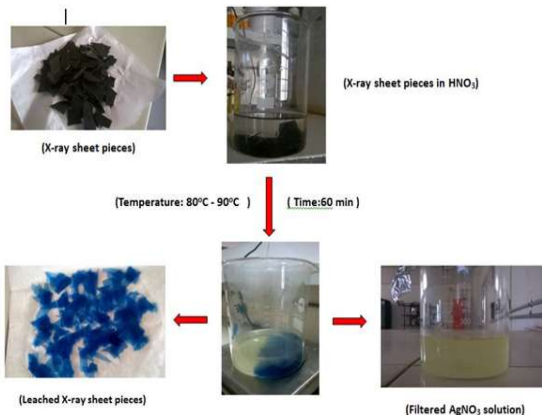
Figure 1: Efficient Silver Nitrate Solution Production from Photographic Films: A Step-by-Step Flowchart
