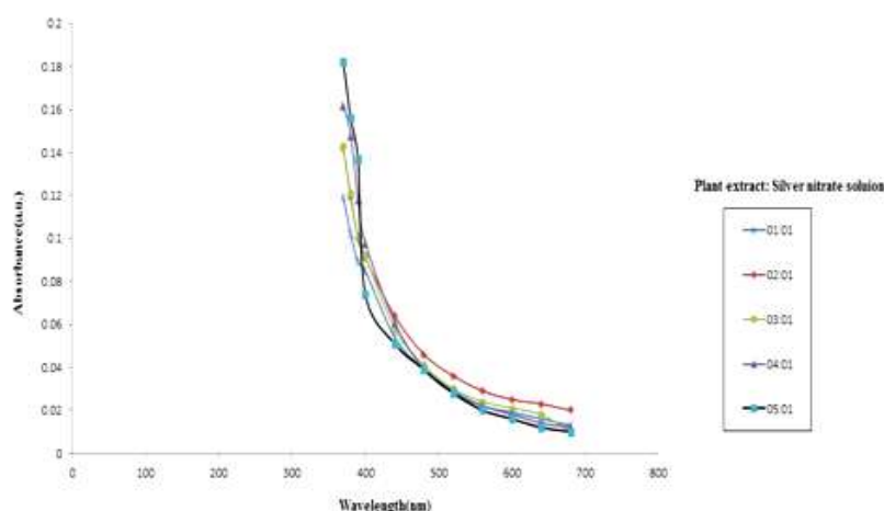
Figure 4: The impact of the Leaf Extract Concentration to Silver Nitrate Solution Ratio on the Synthesis of Silver Nanoparticles
