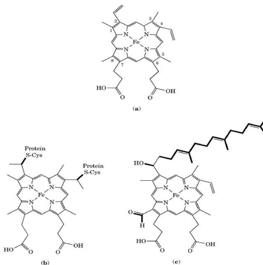
Figure 22: Structures of Cytochromes
