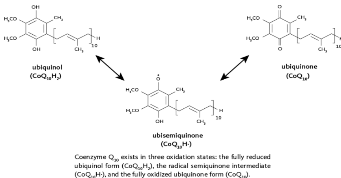
Figure 21: Structures of Coenzymes Q
