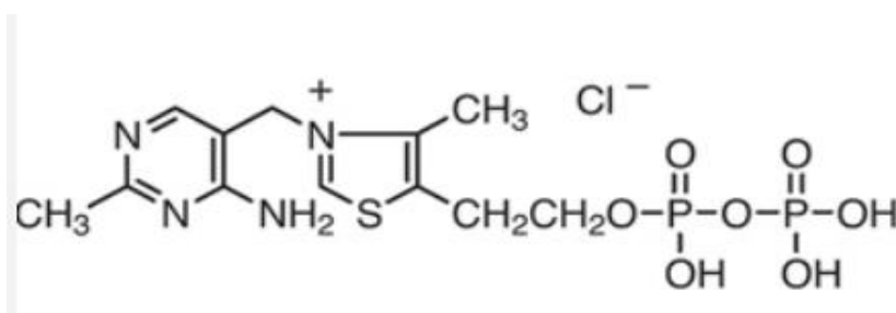
Figure 24: Thiamine Pyrophosphate Chloride
