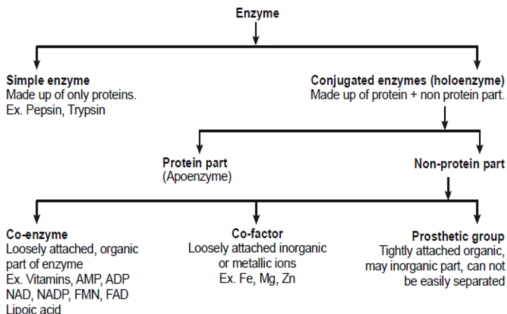
Figure 7: Flowchart of Enzyme Classification
