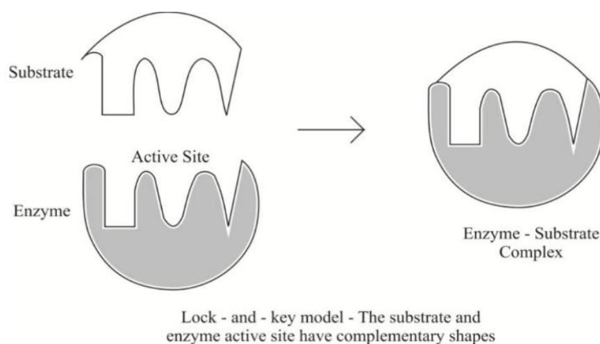
Figure 9: Diagrammatic Representation of Lock and Key Hypothesis
