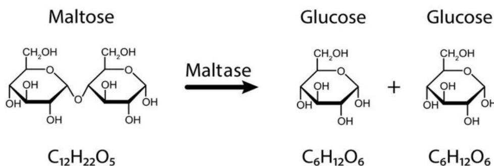
Figure 3: Enzymatic Hydrolysis of Maltose
