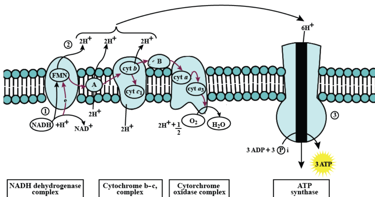
Figure 23: Representation of Electron Transport System
