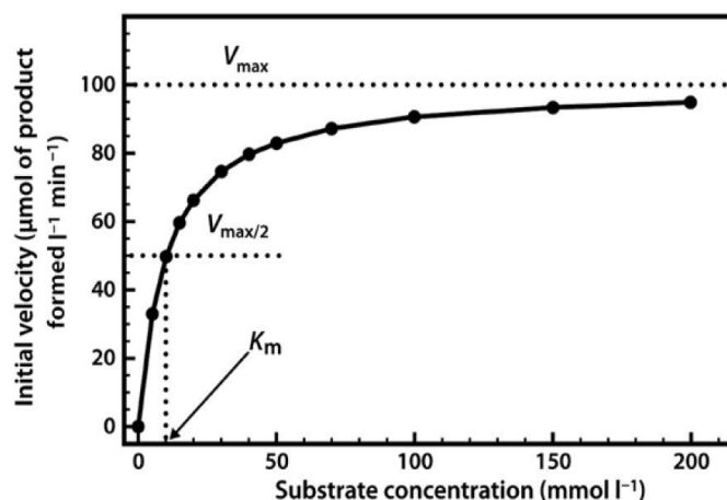
Figure 14: Relation between Substrate Concentration and Rate of an Enzyme-Catalyzed Reaction.
