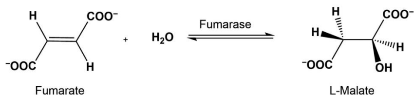
Figure 4: Enzymatic Conversion of Fumarate to Malate
