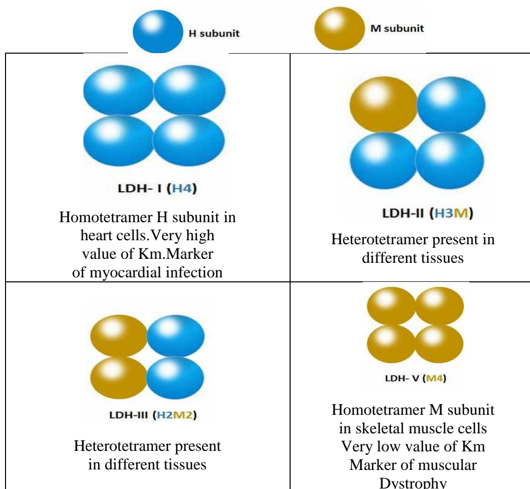
Figure 8: Classification of Tetramers
