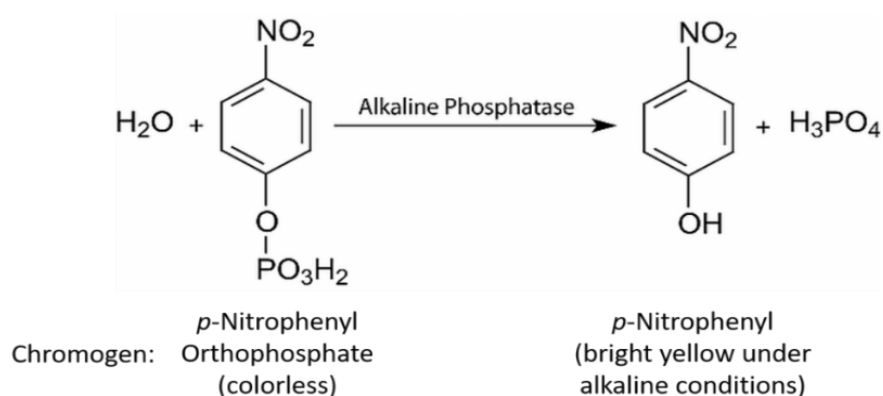
Figure 11: Example of Continuous Assays
