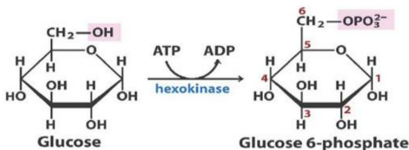
Figure 2: Formation of Glucose- 6- Phosphate from Glucose
