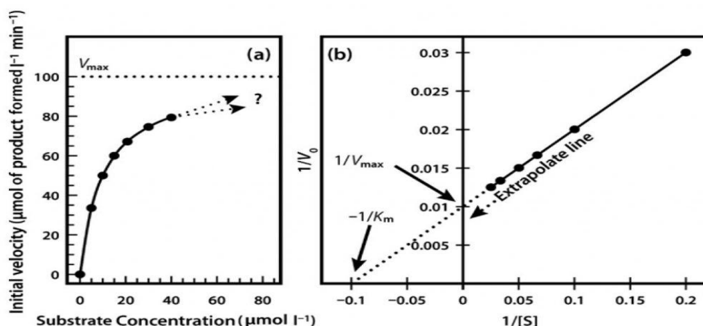
Figure 15: Kinetics of Menton: (i) Direct plot of data (ii) Lineweaver-Burk plot of the same Kinetic Data
