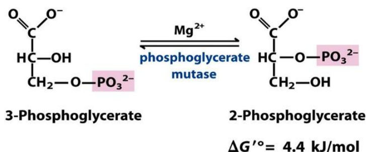
Figure 5: Isomerization by Enzymatic Action
