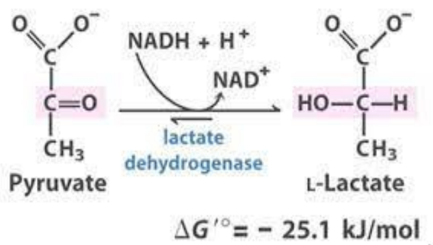
Figure 1: Reduction of Pyruvate to form L- Lactate
