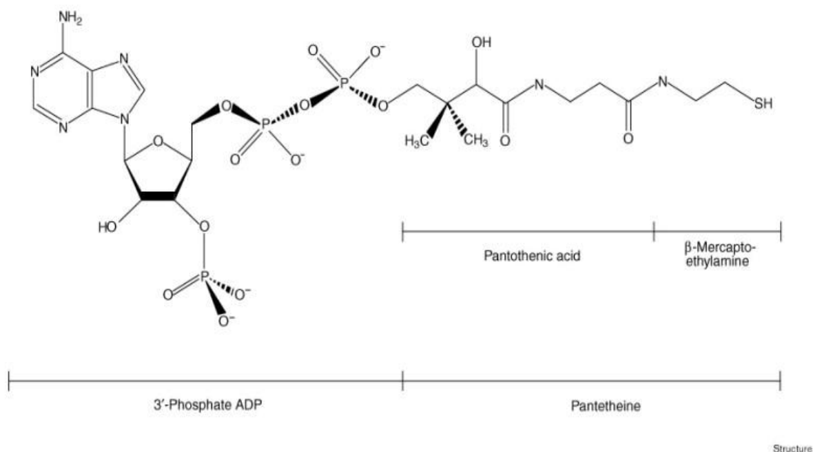
Figure 20: Structure of Coenzyme A
