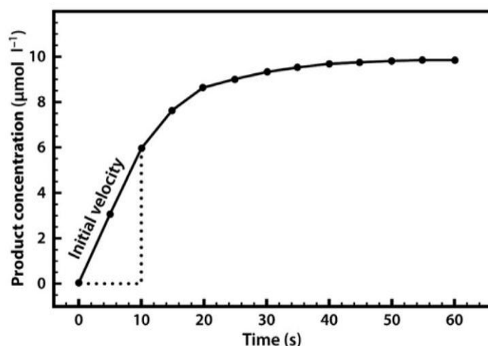
Figure 12: Formation of Product in an Enzyme-Catalyzed Reaction, Plotted Against Time
