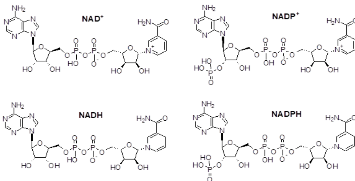
Figure 19: Structure of Pyridine Derivatives
