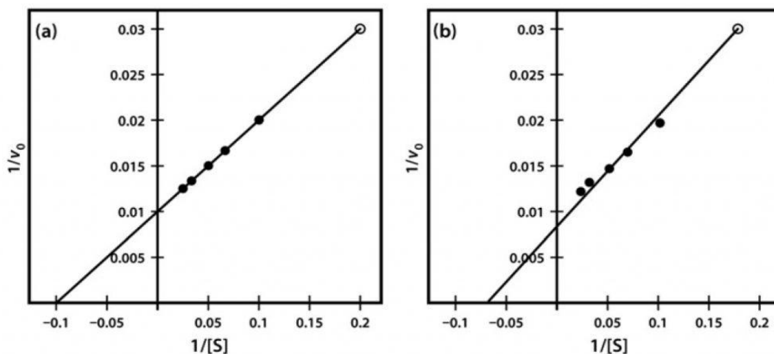
Figure 16: Lineweaver-Burk Plot of Similar Kinetic Data, which differ only in a Single Data Point
