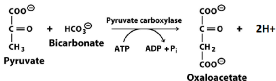
Figure 6: Conversion of Pyruvate to Oxaloacetate by Formation of New Bond
