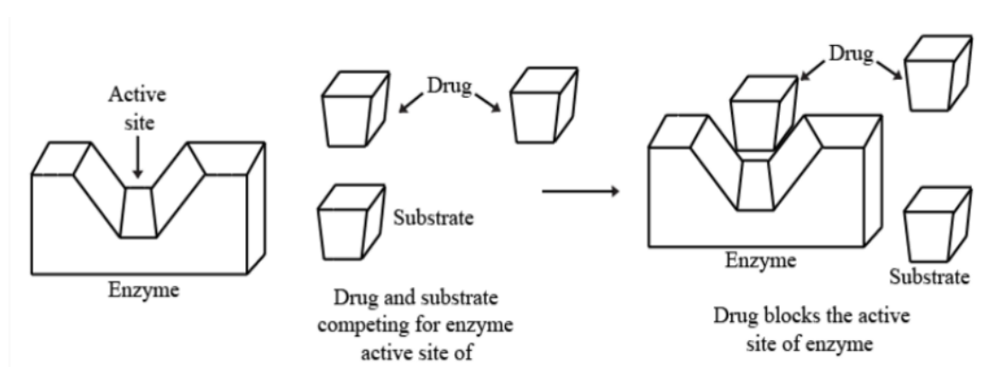
Figure 17: Mechanism of Enzyme Inhibition
