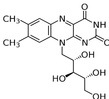
Figure 18: Structure of Riboflavin
