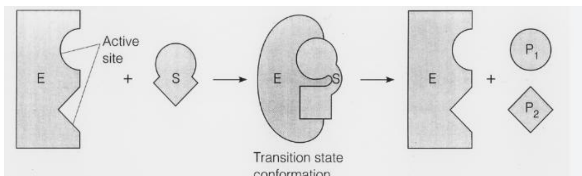
Figure 10: Diagrammatic Representation of Induced Fit Theory
