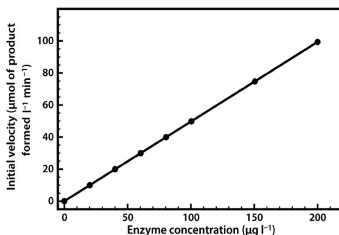
Figure 13: Relationship between Enzyme Concentration and the Rate of an Enzyme-Catalyzed Reaction
