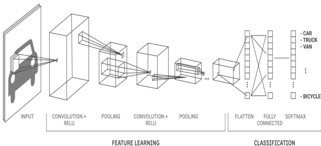
Figure 5: Architecture of a Convolutional Network
