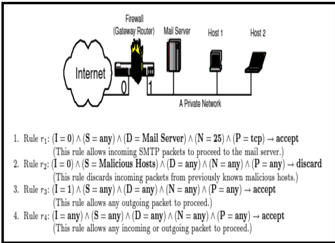
Figure 2: A Firewall Example
