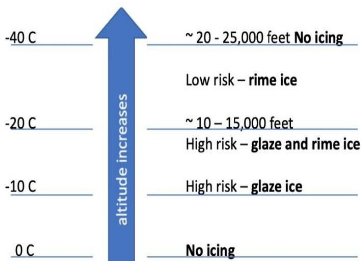
Figure 5: The relationship between altitude, temperature and icing [3].
