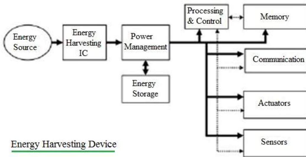
Figure 1: Energy Harvesting Device (Reference 16)
