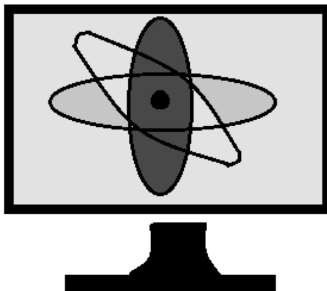
Figure 1: Quantum Computing
