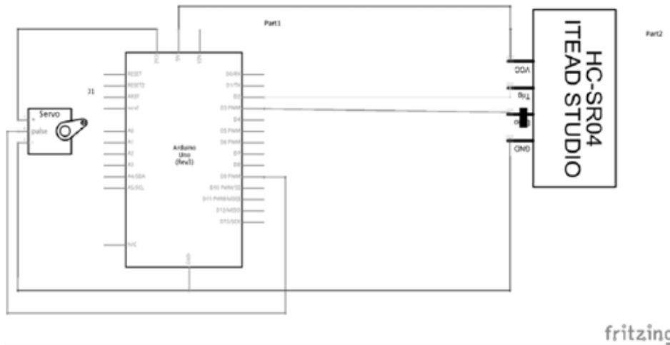
Figure 2: Circuit Diagram of SRP system
