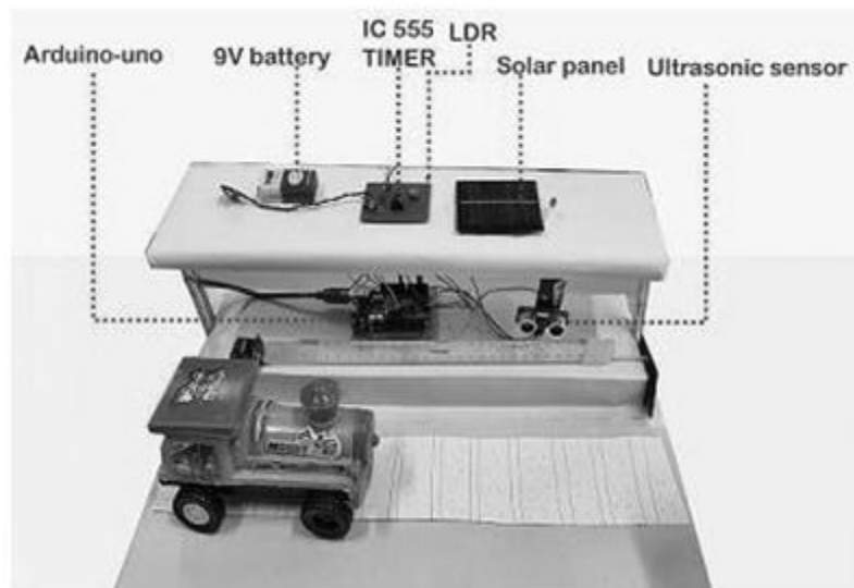
Figure 4: Developed model of the SRP system
