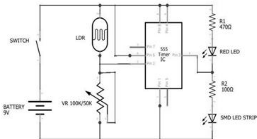
Figure 3: Circuit Diagram of automated Railway Platform Lights
