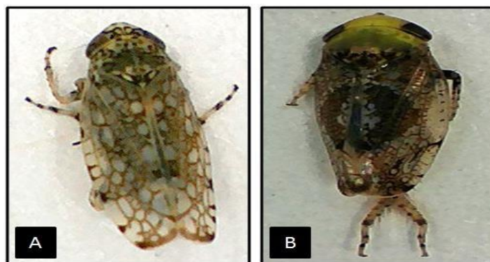
Figure 2: Leafhopper vectors associated with sesamum phyllody disease, A. Orosius albicinctus ; B. Hishimonus phycitis
