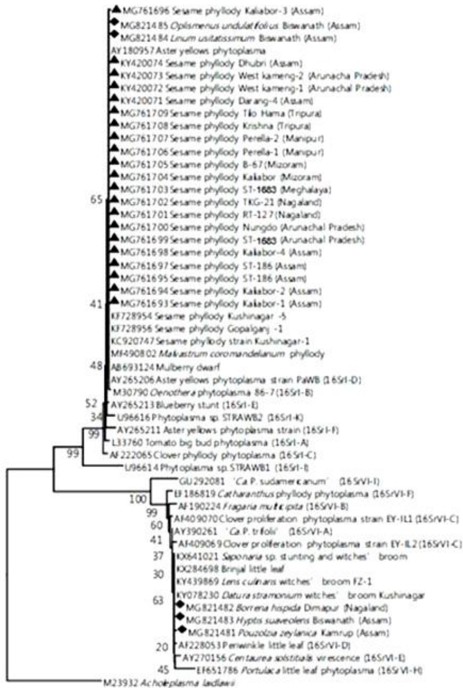
Figure 4: Phylogenetic tree constructed by neighbor-joining method showing the relationships among sesamum phyllody strains and selected phytoplasma strains on 16S rDNA sequences.
