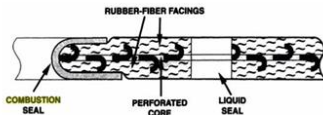
Figure 5: Perforated-Core Head Gasket
