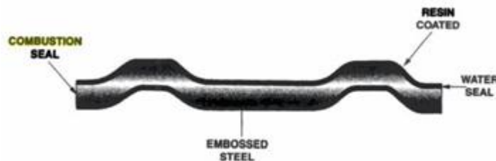
Figure 4: Embossed Steel Shim
