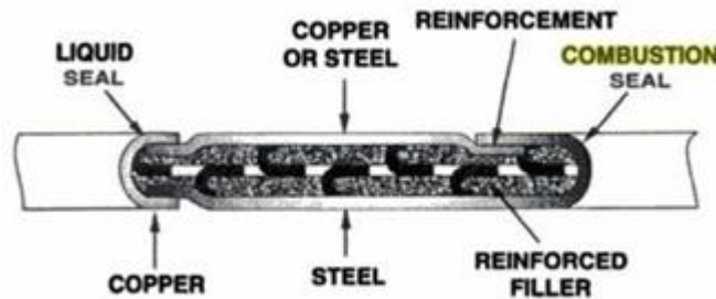
Figure 3: Strengthened Sandwich Gasket
