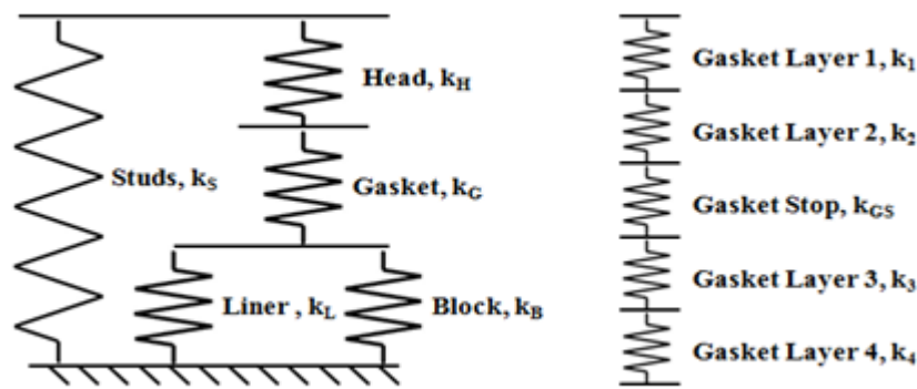
Figure 13(A): Engine Assembly
