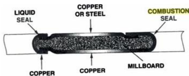
Figure 2: Sandwich gasket
