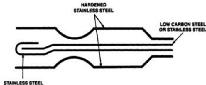
Figure7: Multilayer-Steel Head Gasket
