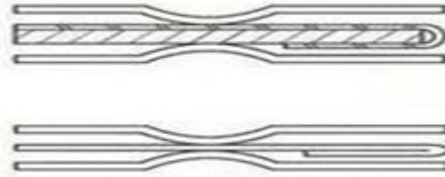
Figure 11: No Obstacle-Type Gasket
