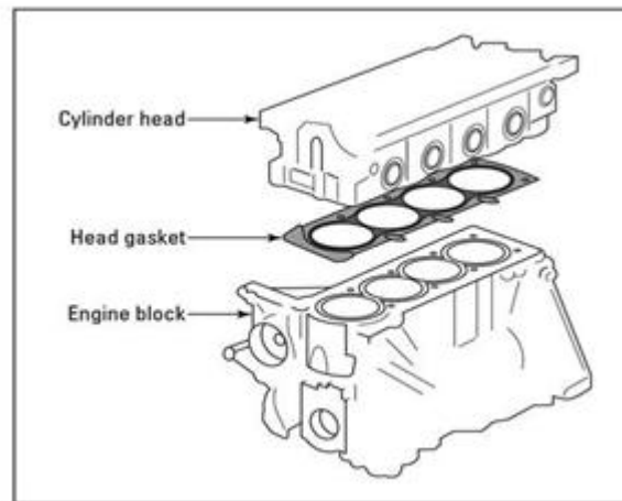
Figure 1: Assembly of Cylinder, Cylinder Head and Gasket
