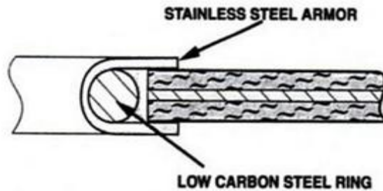
Figure 8 : Stainless Steel Armor with a Steel Ring Head Gasket
