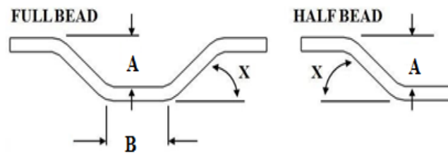
Figure12 (A): Full Bead
