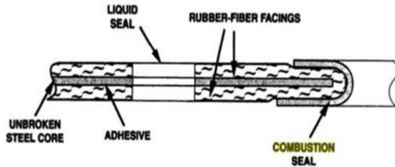
Figure 6: Unbroken-Metal-Core Head Gasket
