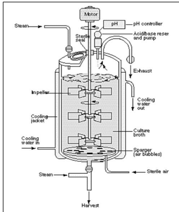
Figure 7: Bioreactor and its components Source : https://biologyease.com/design-of-a-fermentor/
