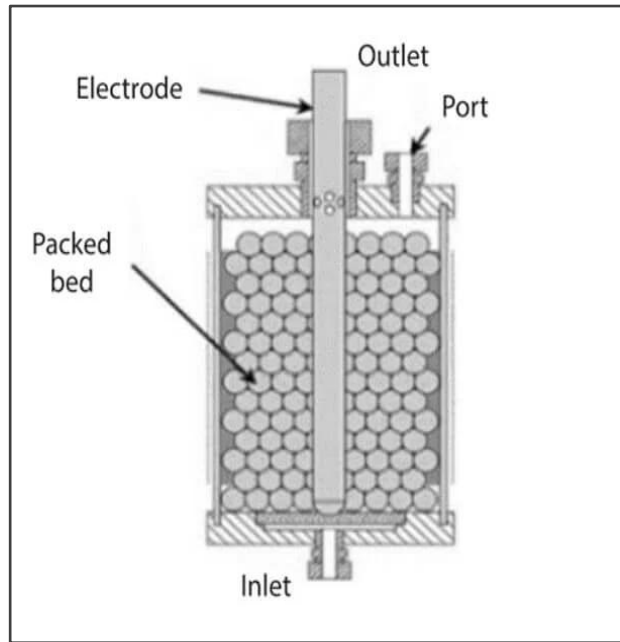
Figure 4: Packed bed fermenter. Image Source: Kuila, A., & Sharma, V. (2018).
