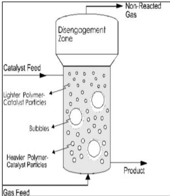
Figure 3: Fluidized bed reactor Image Source: (Kwong W.H, 2000).
