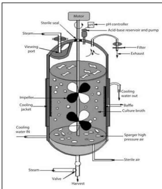
Figure 1: Continuous stirred tank fermenter. Image Source: Saran, S., Malaviya, A., & Chaubey, A. (2019).
