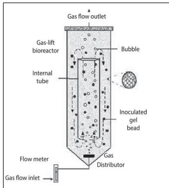
Figure 2: Airlift fermenter. Image Source: Kuila, A., & Sharma, V. (2018).
