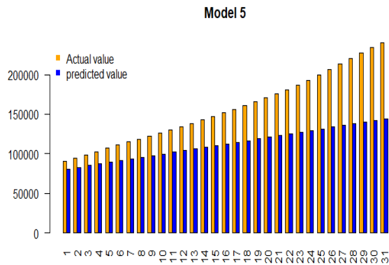
Figure 9: Actual vs. Predicted for lockdown 4 as training and unlock 3 as test dataset
