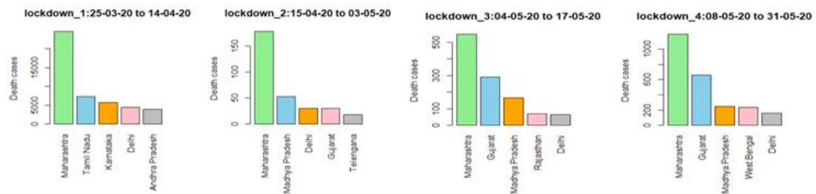
Figure 2: Maximum Affected State with maximum death cases for 4 phases
