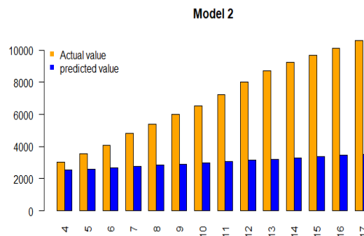
Figure 6: Actual vs Predicted for lockdown 2 as training and lockdown 2 as the test dataset
