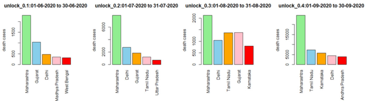
Figure 4: Maximum Affected State with Death cases for Unlock phases
