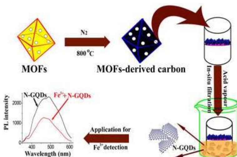
Figure 3: Carbon Dot Synthesis with MOF
