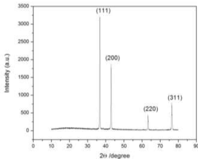
Figure 2: XRD of PAA with MMT
