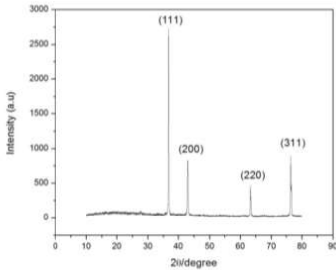
Figure 1: XRD of PAA with KAOLIN
