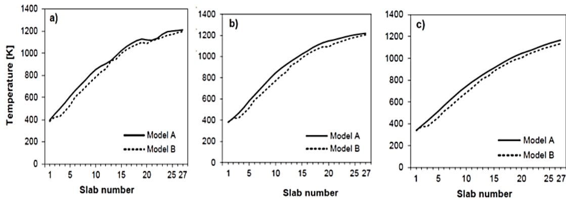
Figure 15: Assessment of mean temperature of slabs in model A and B. (a) top surface, (b) bottom surface and (c) volume averaged temperature[6].
