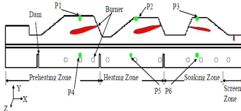
Figure 9: Schematic of WB Furnace Showing Temperature Measurement Points( P_i )[13]
