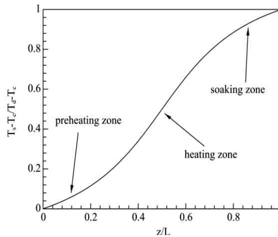
Figure 18: Representative Arctangent Curve for Slab Surface Temperature in Reheating Furnace[51]
