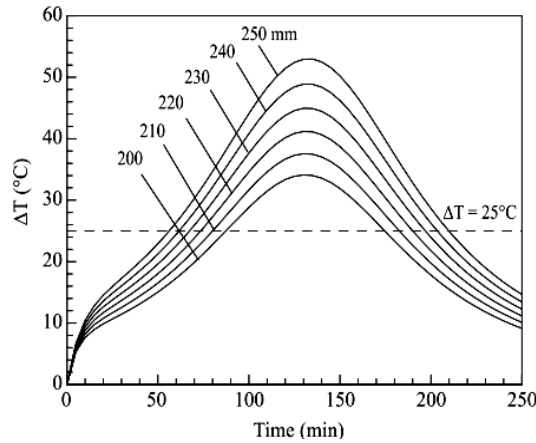
Figure 21: Effect of Slab Width Fixed at 1250 Mm on Temperature Uniformity at Various Slab Gauges[51]
