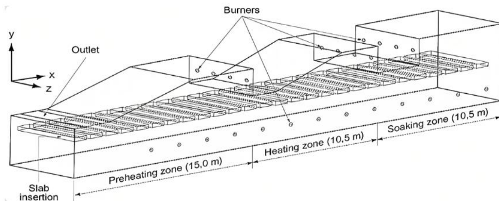
Figure 2: Schematic of Walking Beam Type Reheating Furnace(WB furnace) without Skid Beam Arrangement[6]
