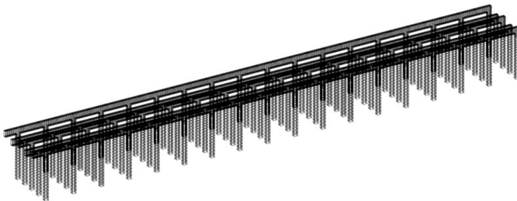
Figure 4: Mesh of skid post and skid beam systems[16]
