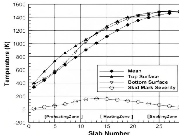
Figure 11: Temperature profiles of slab and skid mark severity [15]
