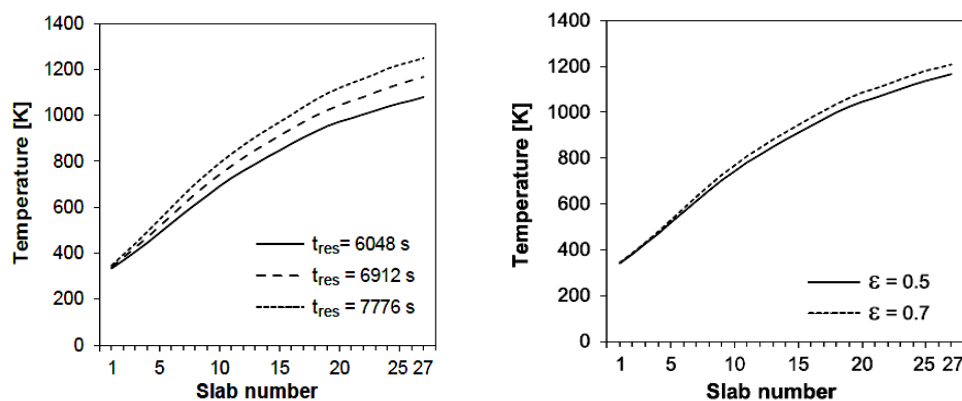
Figure 16: Influence of (a) residence time and (b) slab emissivity on slab's average temperature profile along length of reheating furnace[6].
