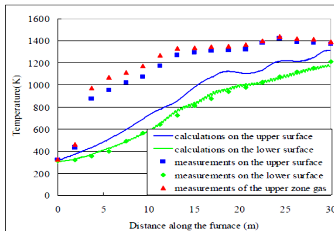
Figure 10: Temperature variation along central lines on top and bottom surfaces of slab [13]
