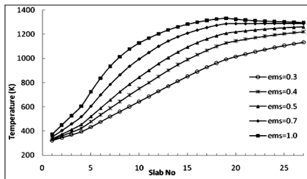
Figure 14: Slab emissivity's effect on the volume-averaged temperature of the slabs with constant furnace medium absorption coefficient ( 1.0 \text{ m}^{-1} ) and furnace wall emissivity (0.75) [18]
