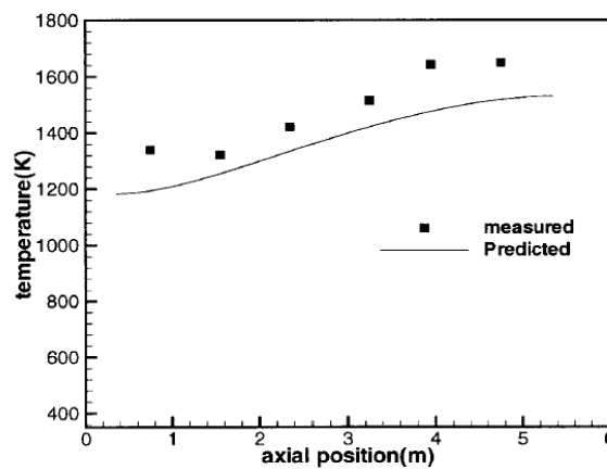
Figure 6: Comparison between measured and predicted temperatures in simplified burner [11]
