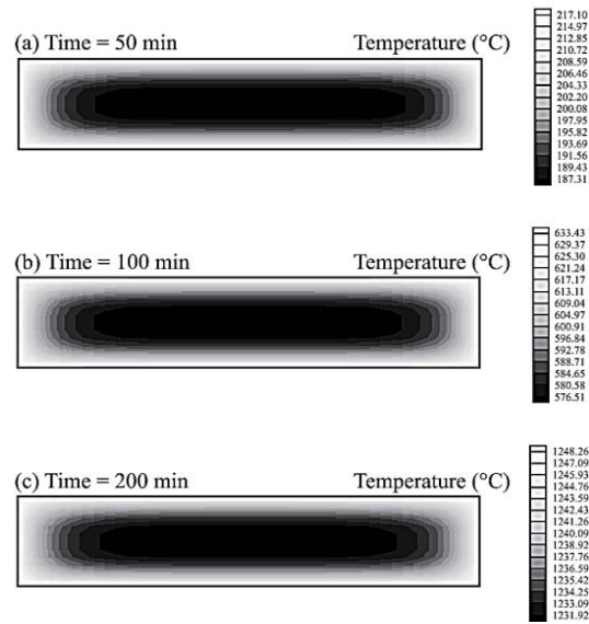
Figure 19: Isothermal Contours Inside Slab at Various Holding Time[51]
