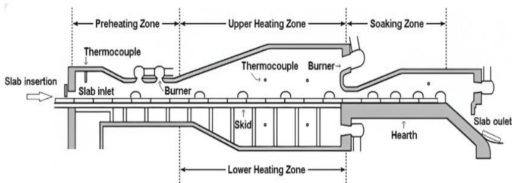
Figure 1: Schematic of Pusher Type Reheating Furnace[5]
