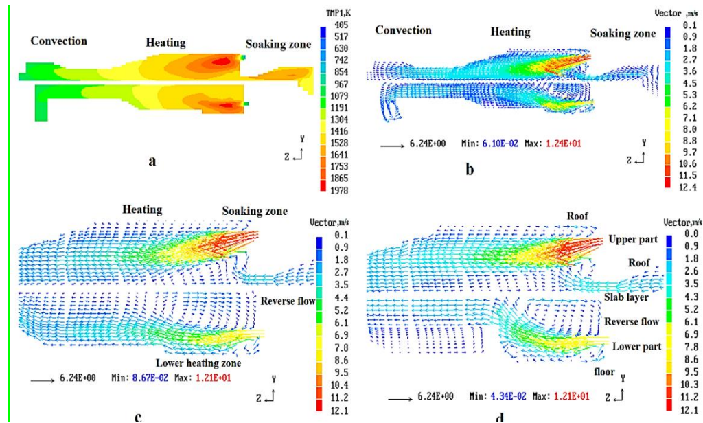
Figure 8: (a) Gas temperature variation, and (b) hot gaseous flow pattern in longitudinal direction; and velocity variation of gaseous flow near burner in heating and soaking zone of the (c) without and (d) with block wall[36]
