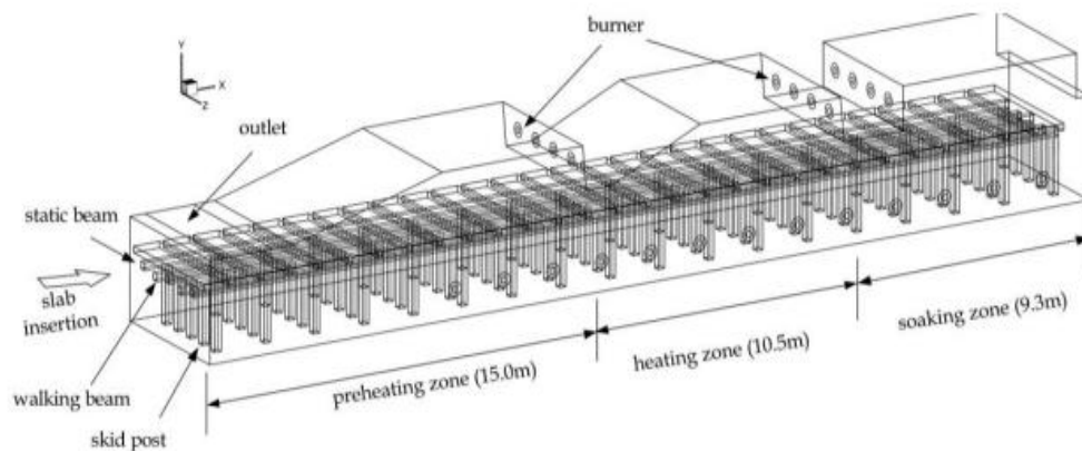
Figure 3: Configuration of the WB furnace, with axial and side burners in the upper and lower zones, respectively, on skid post and skid beam systems[16].
