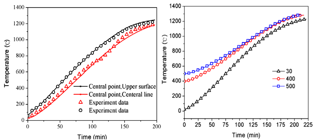
Figure 12: (a) Slab surface and central line temperature (b) Influence of slab lower temperature on different charging temperatures[17]
