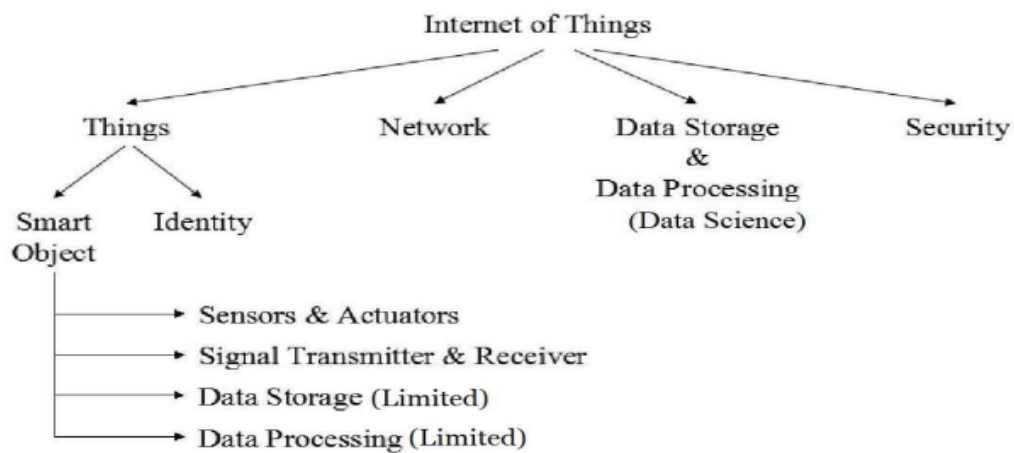
Figure 1: IoT Tree Architecture
