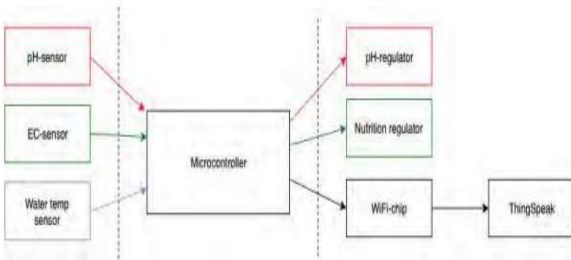
Figure 5: Block diagram
