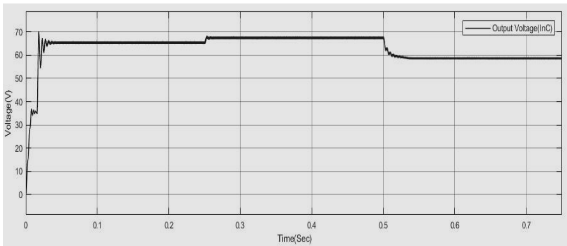
Figure 16.a: Output Voltage (Inc) of PV for Various Irradiance And Constant Temperature 25°C
