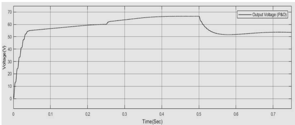
Figure 17.a: Output Voltage (P&O) of PV for Various Irradiance and Constant Temperature 25°C
