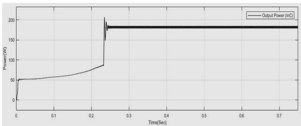
Figure 13: Output Power of Incremental Conduction at 1000\text{W/m}^2 and constant temperature( 25^\circ\text{c} )
