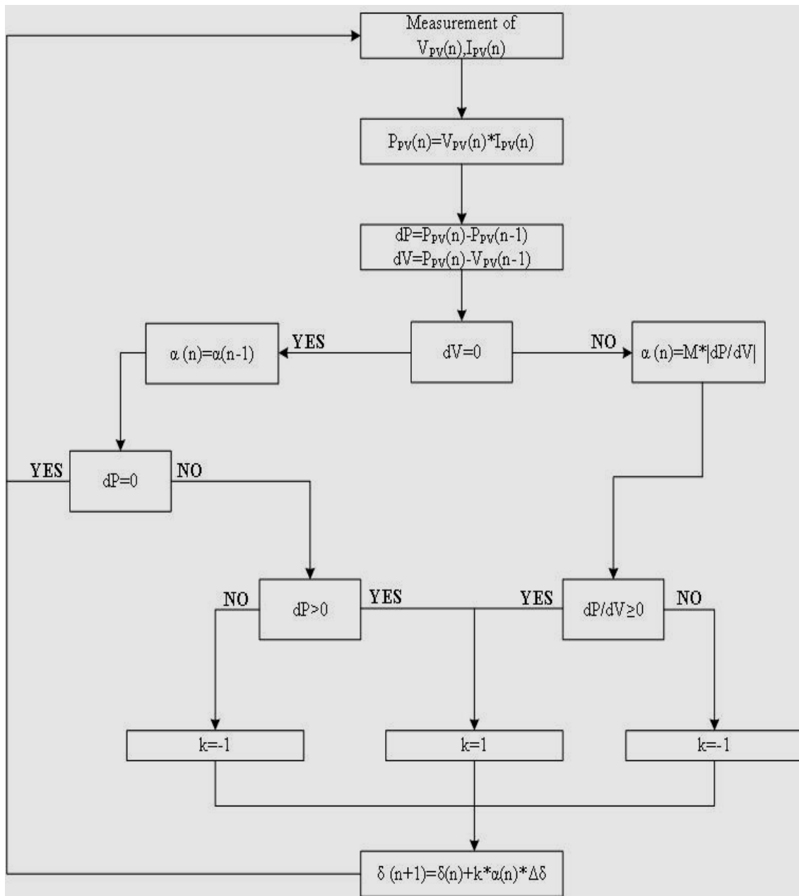
Figure 8: P&Ob Method's Flow Chart
