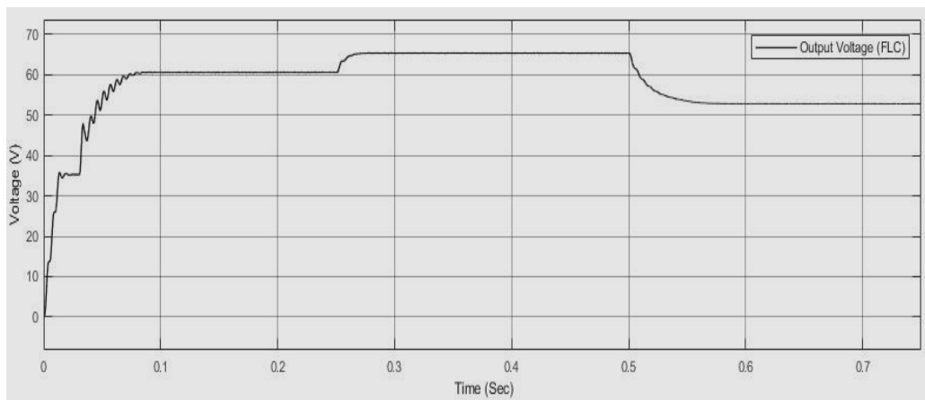
Figure 18.a: Output Voltage (FLC) of PV for Various Irradiance and Constant Temperature 25°C
