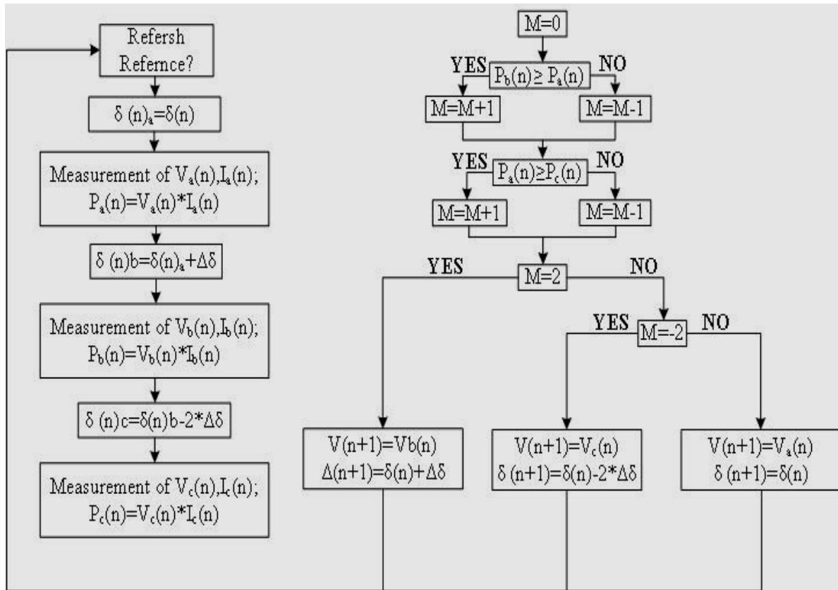
Figure 9: P&O Method's Flow Chart
