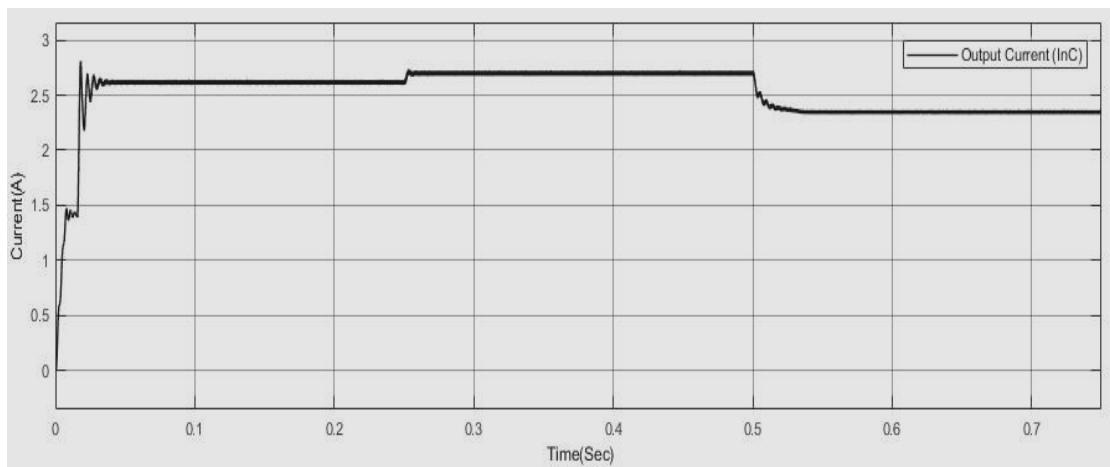
Figure 16.b: Output Current (Inc) Of PV for Various Irradiance And Constant Temperature 25°C
