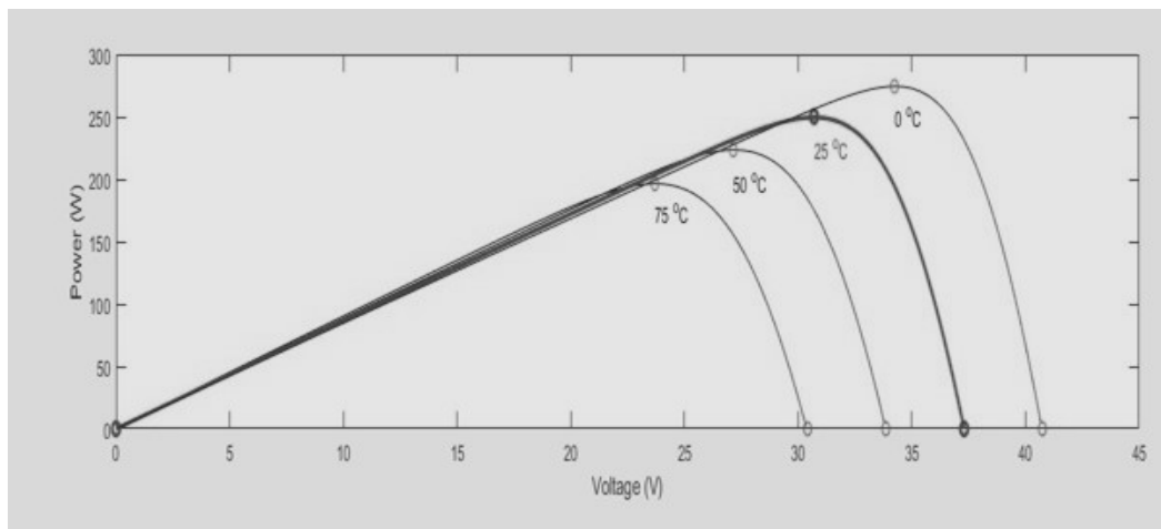
Figure 3: V-P Characteristics of a Photovoltaic Panel for Four Different Temperature Levels
