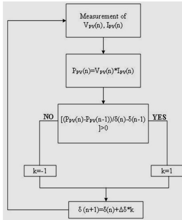
Figure 7: P&Oa Method's Flow Chart
