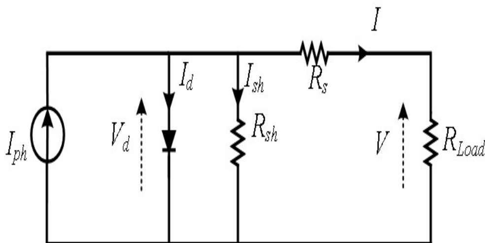
Figure 1: Solar Cell Equivalent Electrical Circuit
