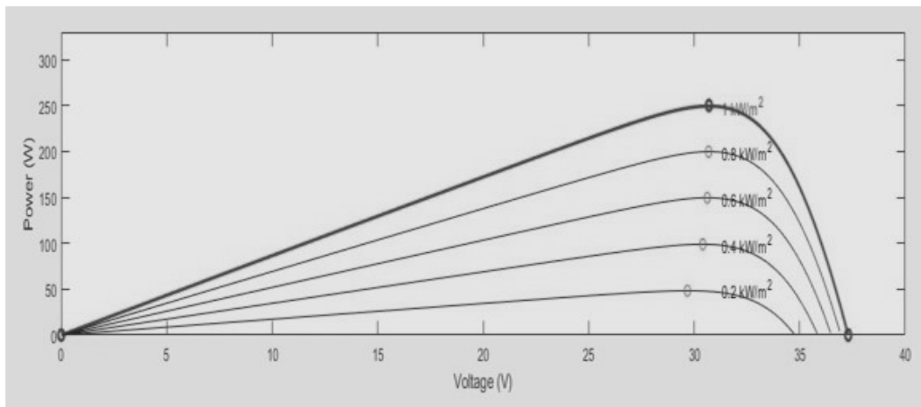
Figure 2: V-P Characteristics of A Photovoltaic Panel For Five Different Irradiance Levels
