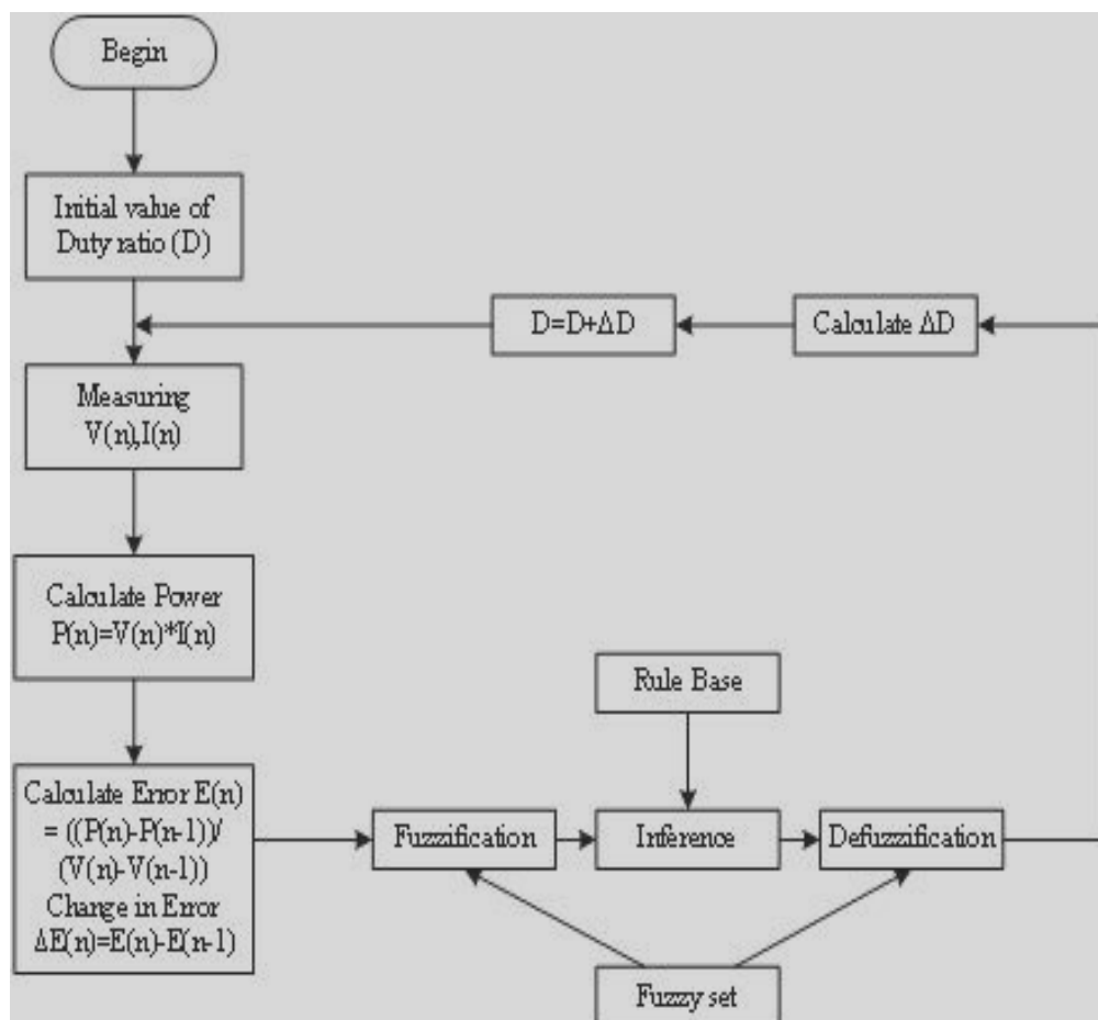
Figure 12: FLC Method's Flow Chart
