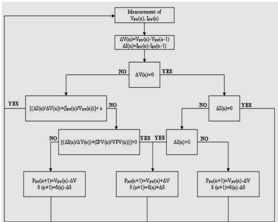
Figure 6: InC Method's Flowchart
