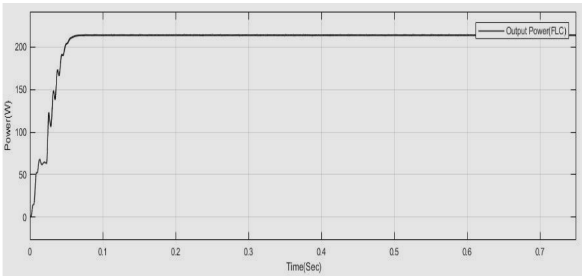
Figure 15: Output Power of Fuzzy Logic Controller At 1000W/M 2 And Constant Temperature(25°C)
