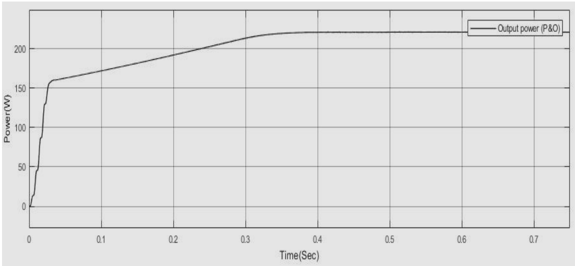
Figure 14: Output Power of Perturbation and observation(P&O) at 1000W/m 2 and constant temperature(25°C)
