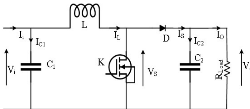
Figure 4: MPPT Boost Converter
