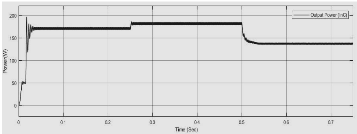
Figure 16.c: Output Power (Inc) Of PV For Various Irradiance And Constant Temperature 25°C
