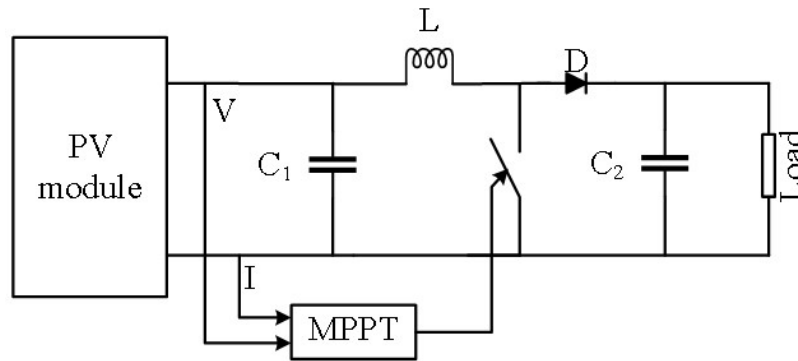
Figure 5: PV system with DC-DC Boost Converter, MPPT
