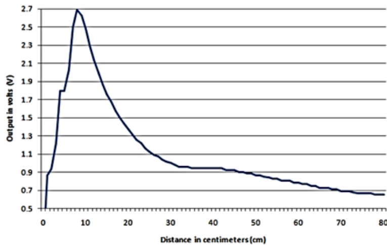
Figure 4: Distance Measurement with respect to voltage
