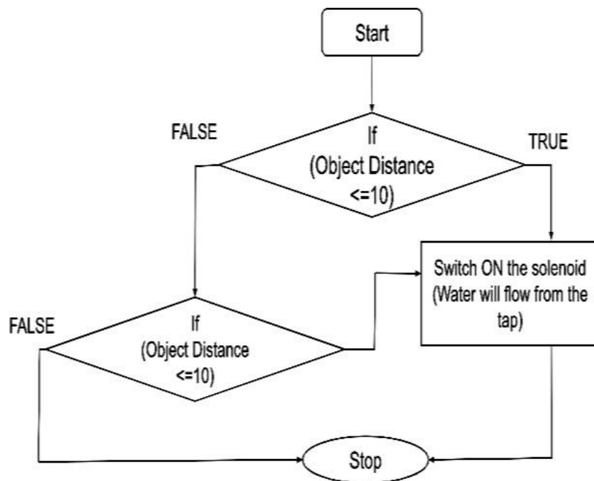
Figure 2: Flowchart of Water Tap
