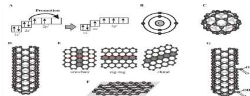
Figure 6: Structure of carbon atom and Carbon based Nanomaterials
