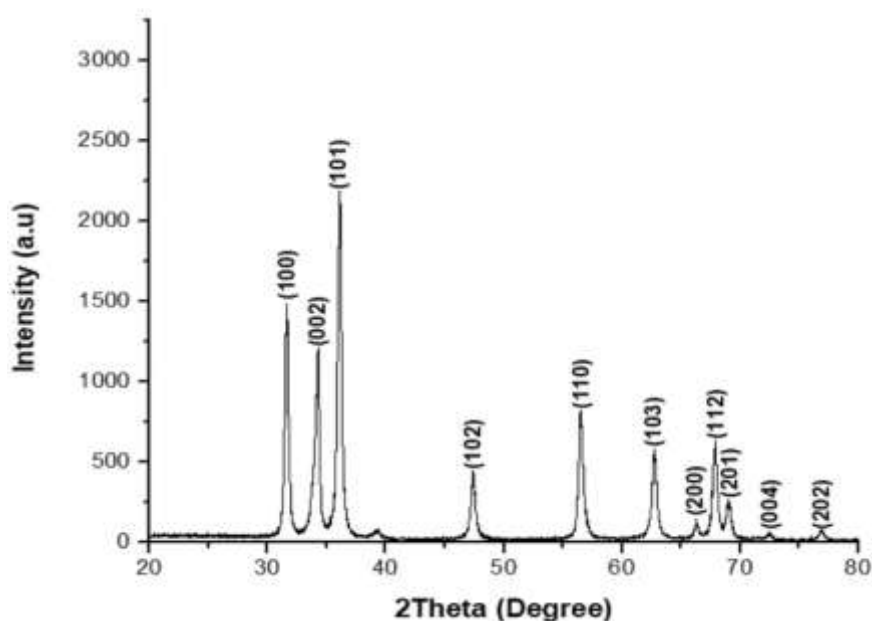
Figure 17: Sample XRD Peak intensities at various \Theta values
