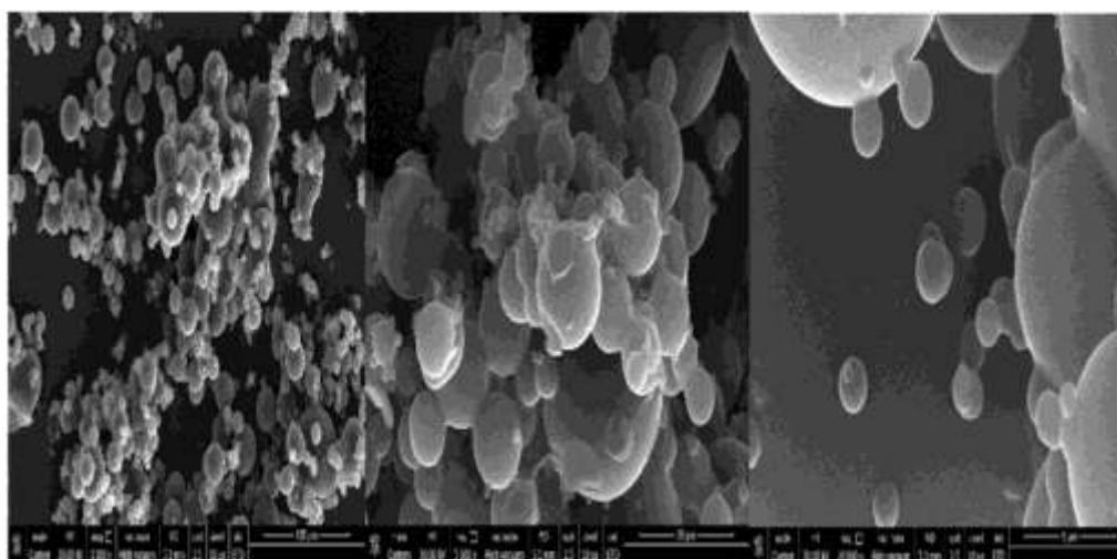
Figure 16: Sample SEM images of Zinc Nanoparticles (a) 1000X Mag. (b) 5000X Mag (c) 20,000X Mag.
