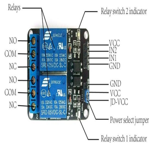
Figure 3: 2-channel relay
