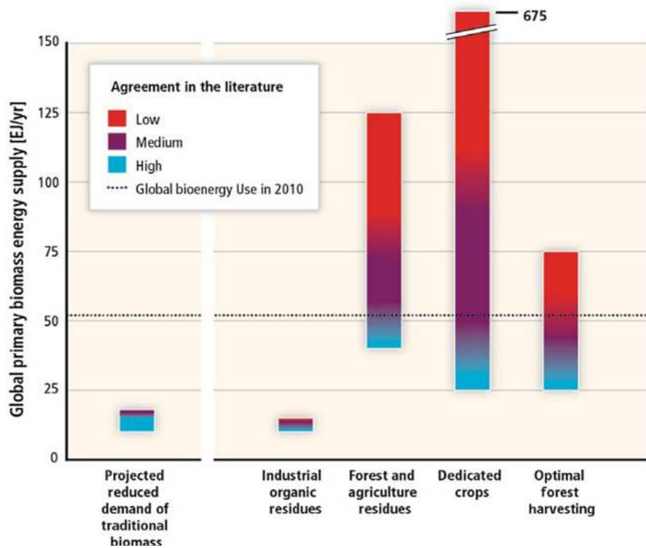
Figure 3: Technical Primary Biomass Potential for Bioenergy on a Global Scale by Main Resource Category in 2050. The worldwide technical primary biomass potential for bioenergy is depicted in the figure along with the estimation ranges for each main resource type. From blue (all researchers believe that this level can be obtained), through purple (medium agreement), to red (few researchers agree that this level can be attained), the color grading is meant to qualitatively demonstrate the degree of agreement in the estimations. Additionally, lowering the need for conventional biomass by improving its efficiency might free up the conserved biomass for alternative energy uses, which would have a significant positive impact on sustainable development [34]
