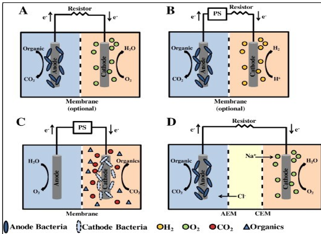
Figure 6: Basic principles in four typical MESS (left chamber: anode; right chamber: cathode). (A) Electricity generation in air-cathode microbial fuel cells (MFCs); (B) hydrogen generation with external power supply in microbial electrolysis cells (MECs); (C) chemical production by microbial electrosynthesis (MES); (D) middle chamber desalination in microbial desalination cells (MDCs). [15]
