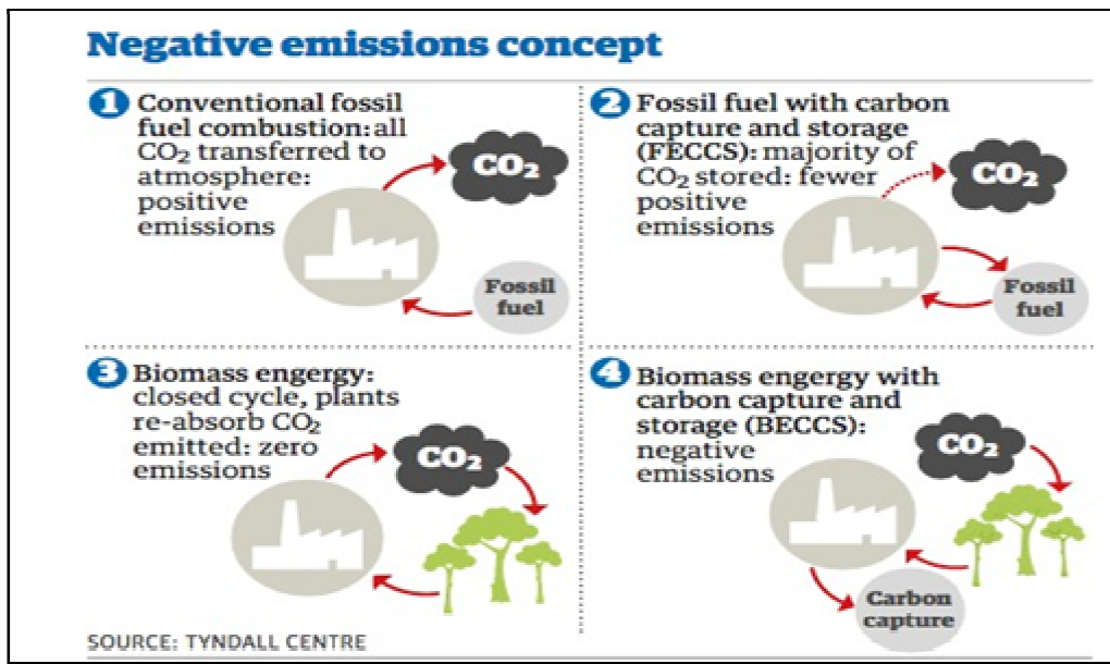
Figure 7: Visualization of Negative Emission Concept
