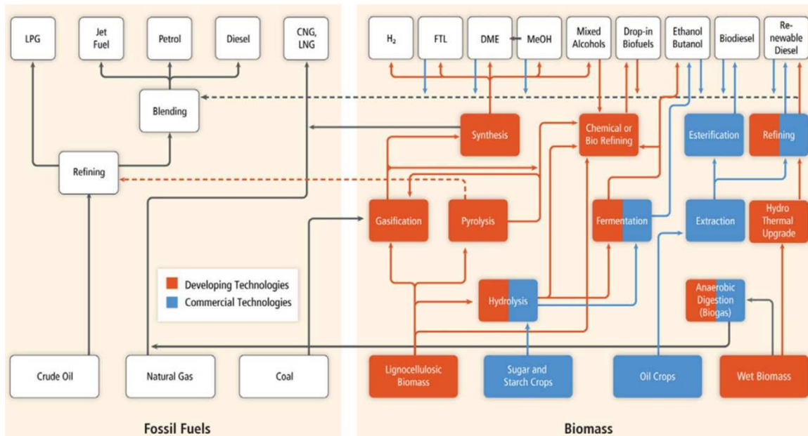
Figure 2: Production Pathways to Liquid and Gaseous Fuels from Biomass and, for Comparison from Fossil Fuels [33]
