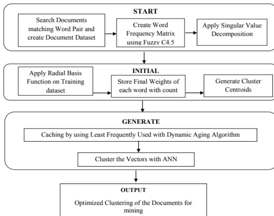
The process of organizing unstructured data and how it flows
