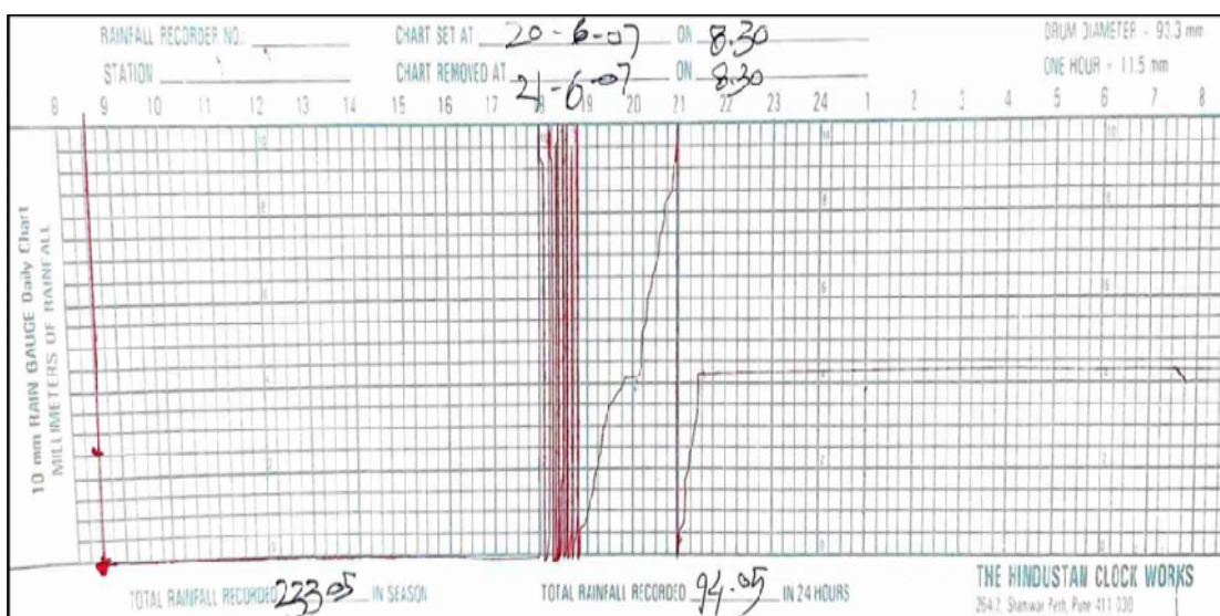
Figure 2: Analysis of Continuous Type Rain gauge Chart
