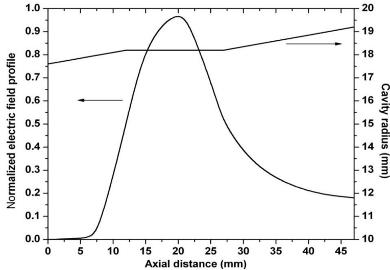
Figure 2: Electric Field Profile of the Cavity
