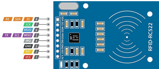
Figure 1: Pin Diagram of Module : RFID-RC522
