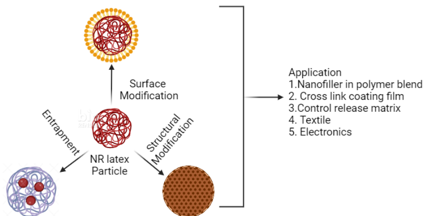
Figure 3: Natural rubber latex's versatility in the field of medical, biological and applied science.
