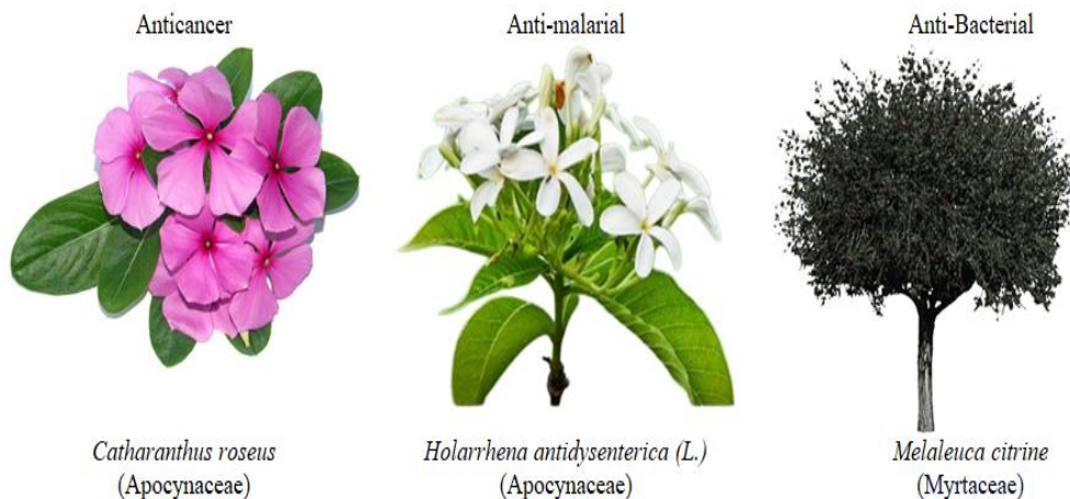
Figure 1: Different plants and its clinical application
