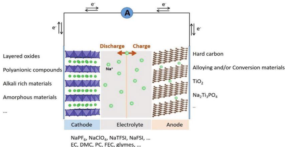
Figure 4: Schematic of sodium-ion battery
