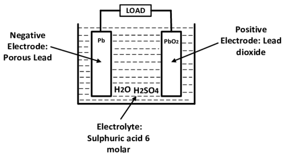
Figure 1: Lead acid battery
