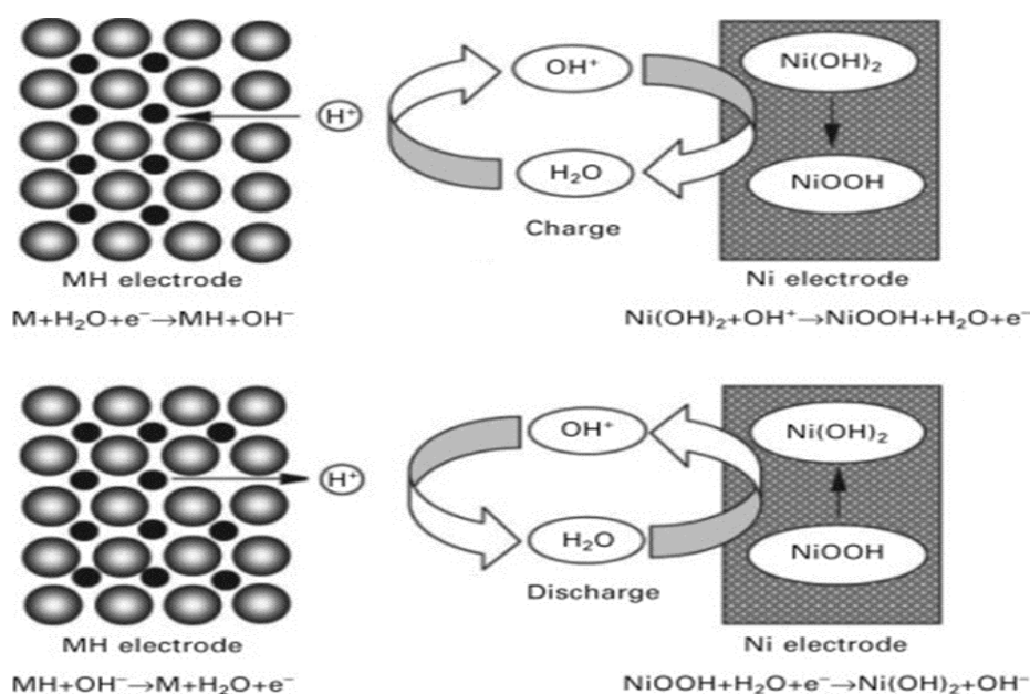
Figure 2: Nickel Metal Hydride battery overview
