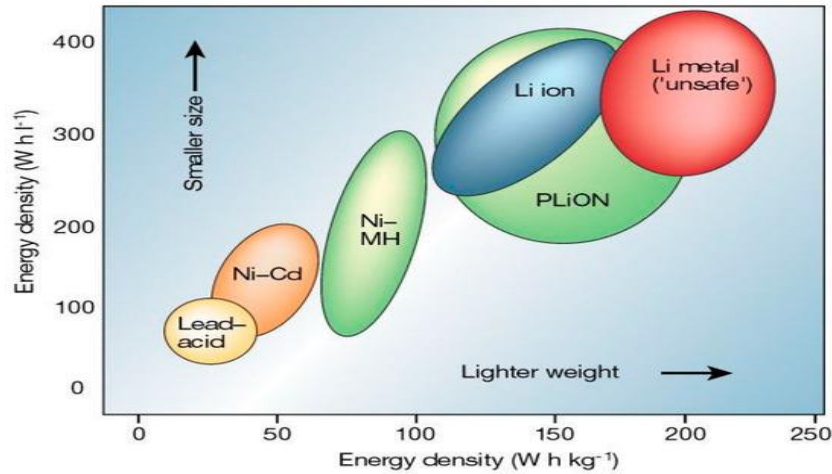
Figure 7: Battery technologies used in EVs
