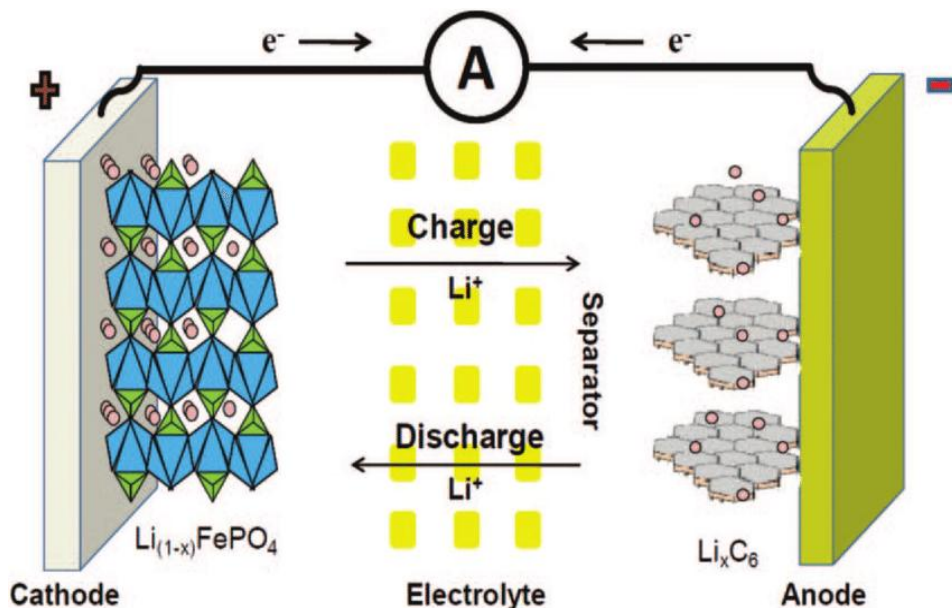
Figure 3: Schematic of Lithium-ion battery
