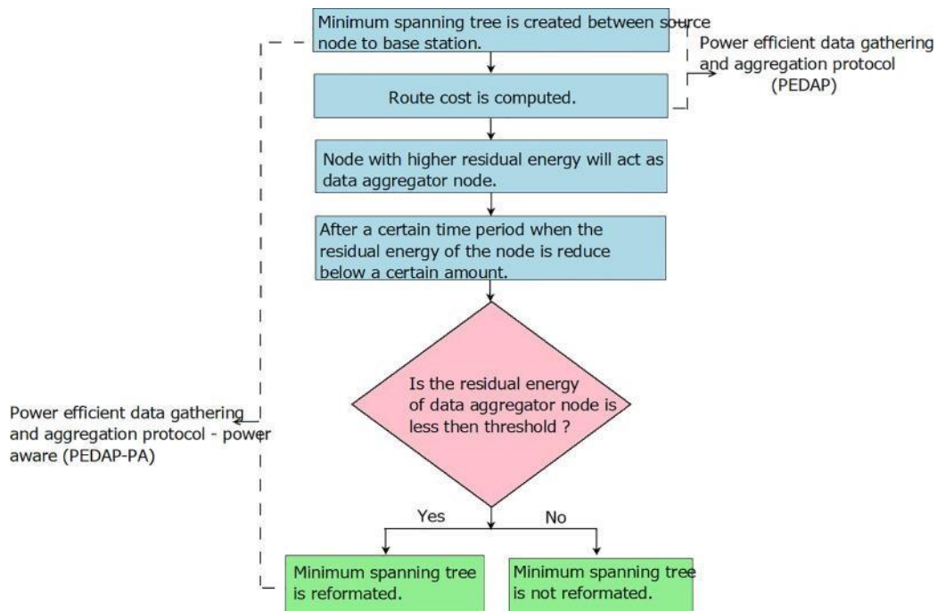
Figure 1: Schematic Diagram of Data Aggregation
