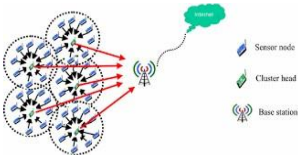
Figure 3: Schematic diagram for Energy Efficient Algorithm
