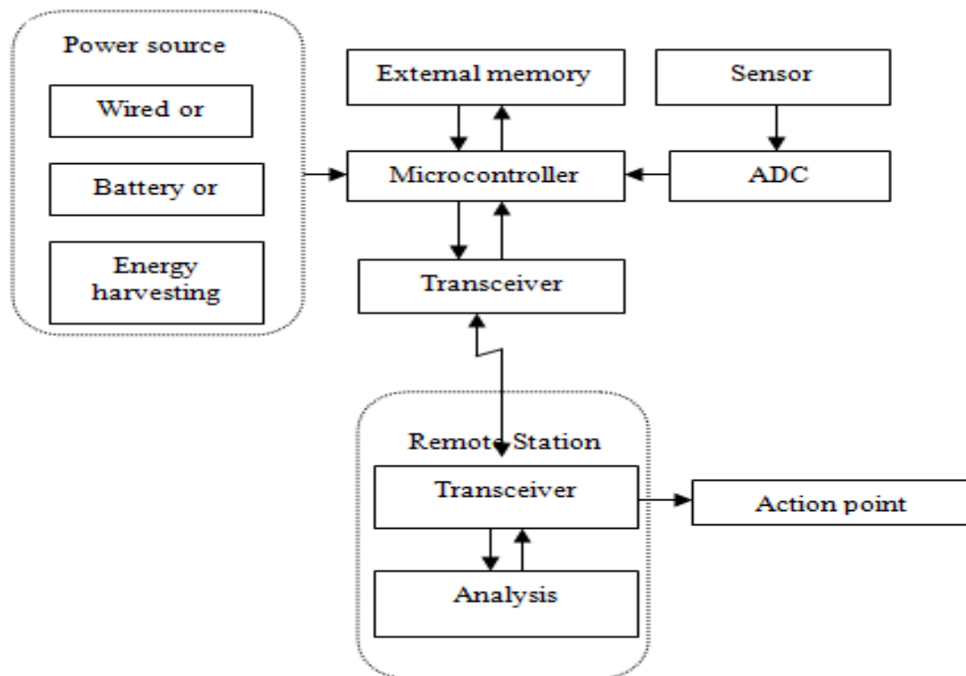
Figure 4: Block Diagram of wireless Sensor Node communication channel.
