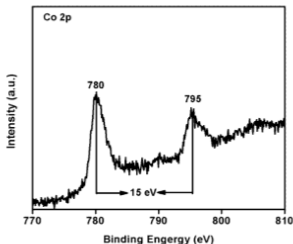
Figure 4: (e) XPS spectra of Co_3O_4 nanocrystals
