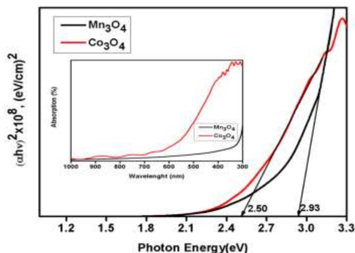
Figure 5: Optical band gaps of Co_3O_4 and Mn_3O_4 nanocrystals
