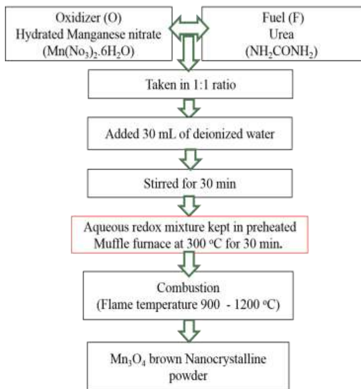
Schematic diagram of solution combustion technique
