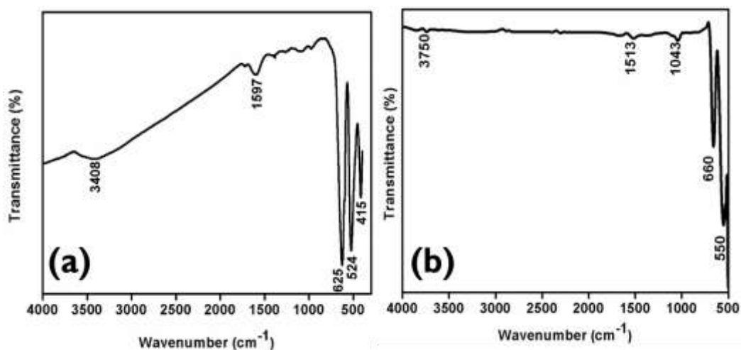
Figure 2: (a) FTIR spectrum of spinel Mn_3O_4 and (b) Co_3O_4
