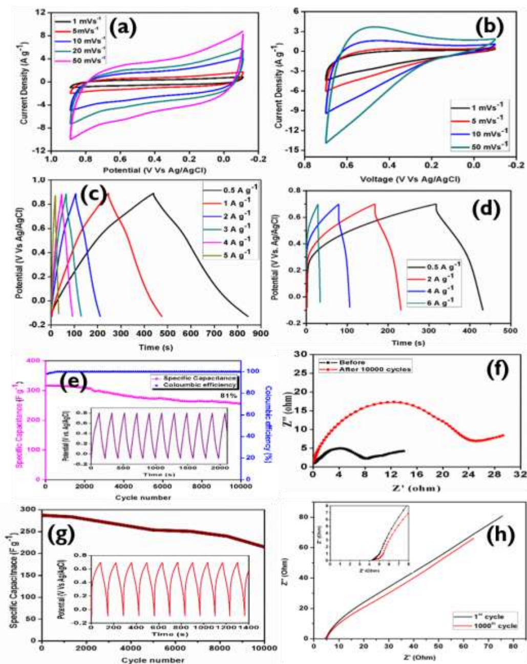
Figure 8: (a) Spinel Mn_3O_4 - cyclic voltammetry curves (b) nanocrystalline Co_3O_4 at various scan rates. (c) Charge-discharge curves of spinel Mn_3O_4 (d) Charge-discharge curves of Co_3O_4 nanocrystals (e) Specific capacitance and coulombic efficacy with cycle number (f) nanocrystalline Mn_3O_4 - Nyquist plots (g) Specific capacitance with cycle number (h) nanocrystalline Co_3O_4 - Nyquist plots
