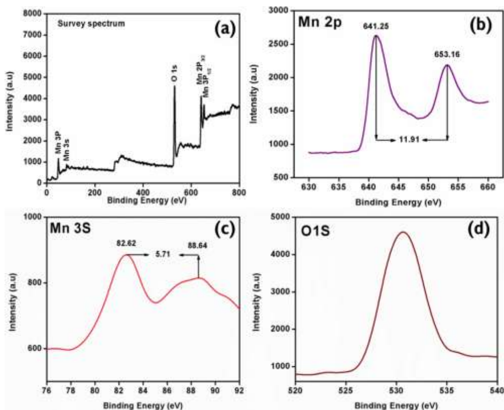
Figure 4: Mn_3O_4 nanocrystals -X-ray Photoelectron spectra (a) Survey spectrum, (b) Mn 2p (c) Mn 3s and (d) O 1s.
