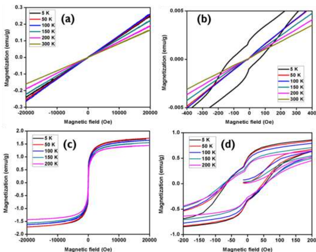
Figure 6: (a & b) M–H curves of Mn 3 O 4 and (c & d) Co 3 O 4 nanocrystals at 5K to 300 K.
