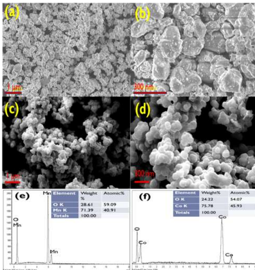
Figure 3: (a & b) SEM images of spinel Mn_3O_4 and (c & d) Co_3O_4 nanocrystals EDS of spinel (e) Mn_3O_4 (f) Co_3O_4 nanocrystals
