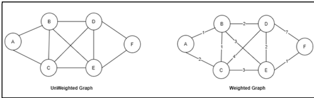
Figure 4: Unweighted and Weighted graph
