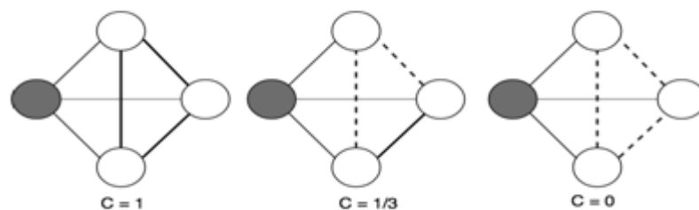
Figure 1: Clustering Coefficient
