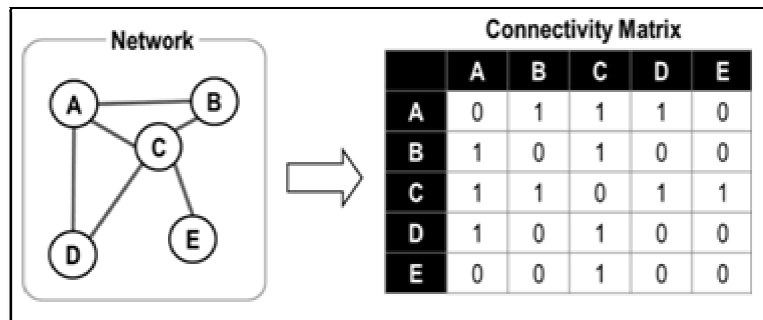
Figure 5: Connection Matrix
