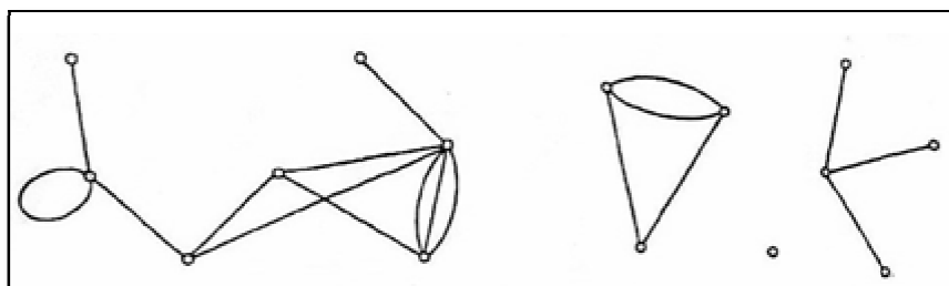
Figure 6: Connected and Disconnected Graph
