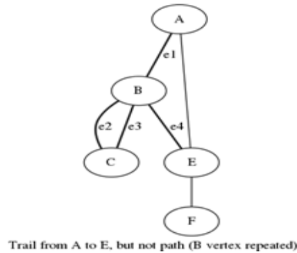
Figure 2: Path Length
