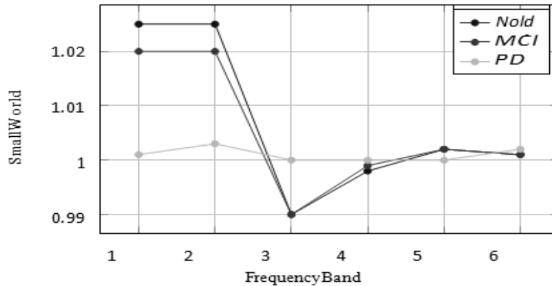
Figure 10: [x axis (1asDelta, 2 as Theta, 3 as Alpha1, 4 as Alpha 2, 5as Beta 1, 6 as Beta 2)] Eyes closed
