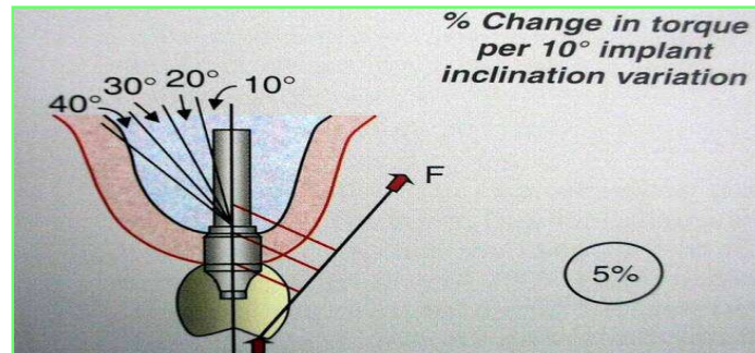
Figure 12: Change in torque per 10-degree implant inclination variation. (27)
