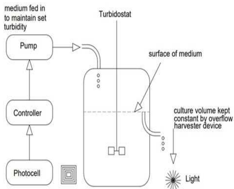
Figure 3: Continuous Fermenter 61
