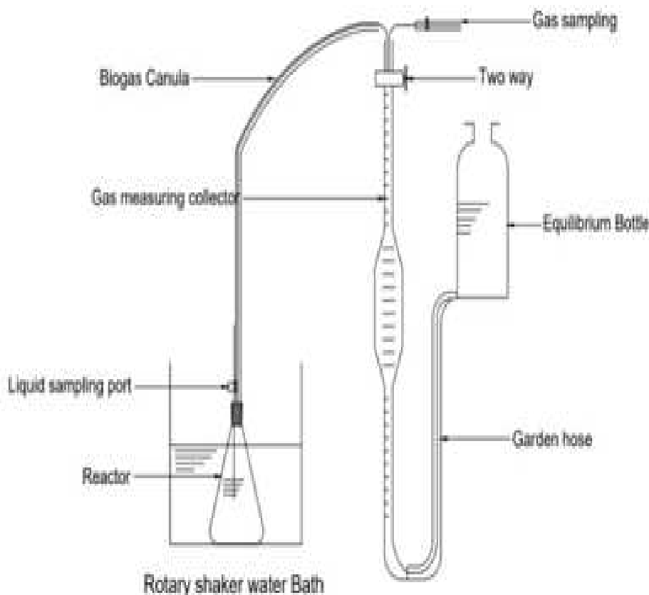
Figure 1: Batch Fermenter 59
