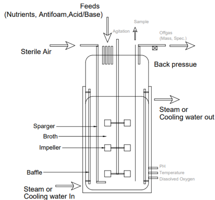
Figure 2: Fed-Batch Fermenter 60
