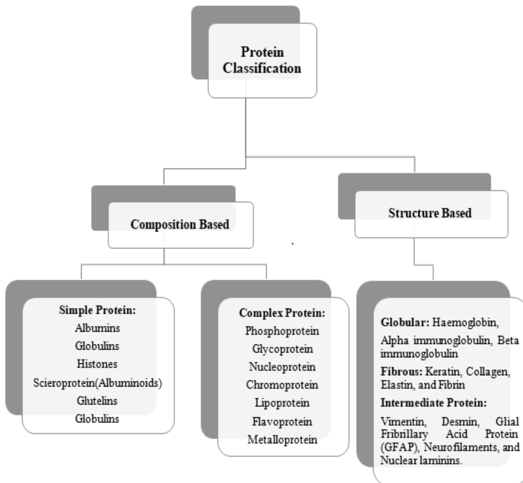
Figure 3: Protein Classification
