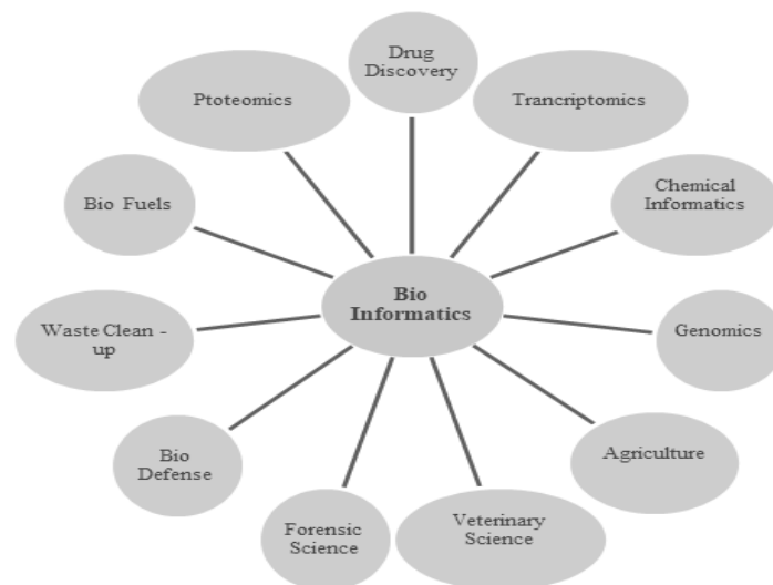
Figure 9: Bioinformatics Applications
