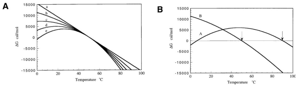
Figure 6: Gibbs Energy
