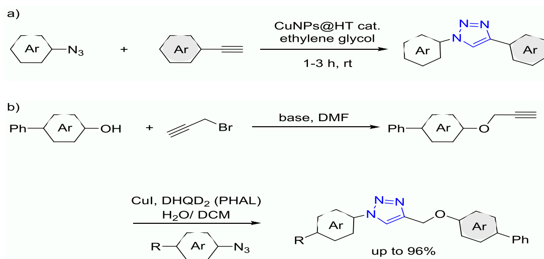
Scheme 1: The 1, 2, 3-triazole synthesis via different catalyst
