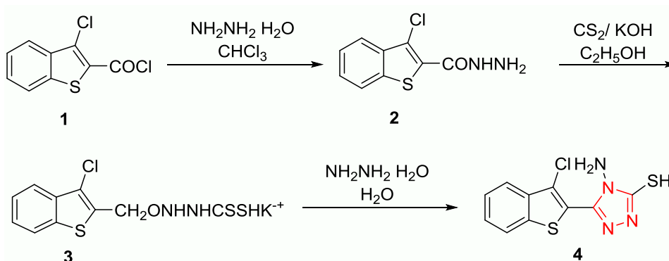
Scheme 8: Synthesis of 1,2,4-triazoles from acid chloride
