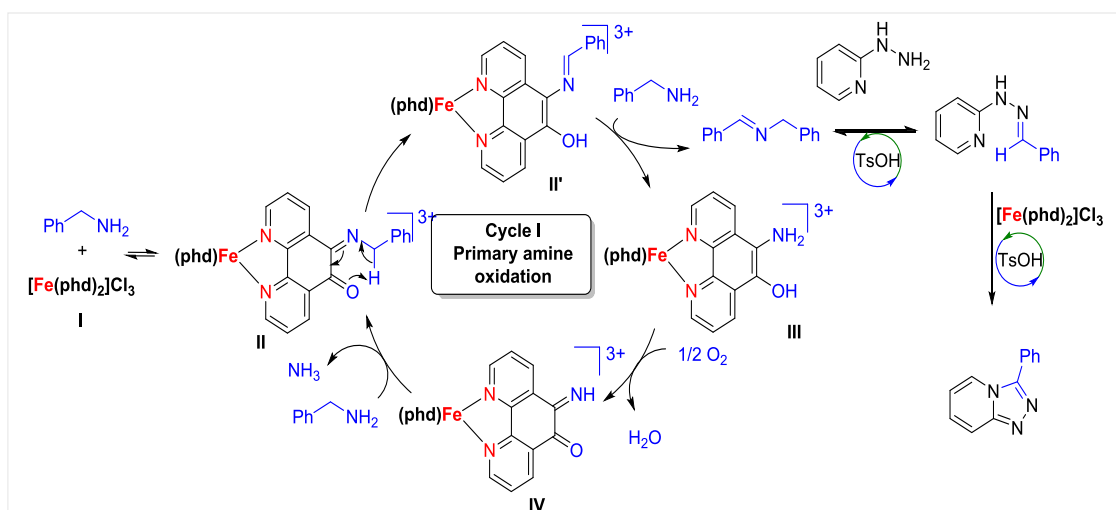
Scheme 7: Bio-mimicking catalytic cycle.
