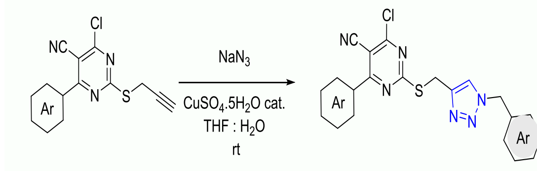
Scheme 4: The 1, 2, 3-triazole synthesis by using the ultrasound technique
