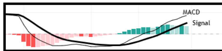
Figure 3: MACD
