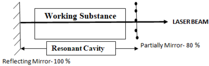
Figure 4: Main Components of a LASER
