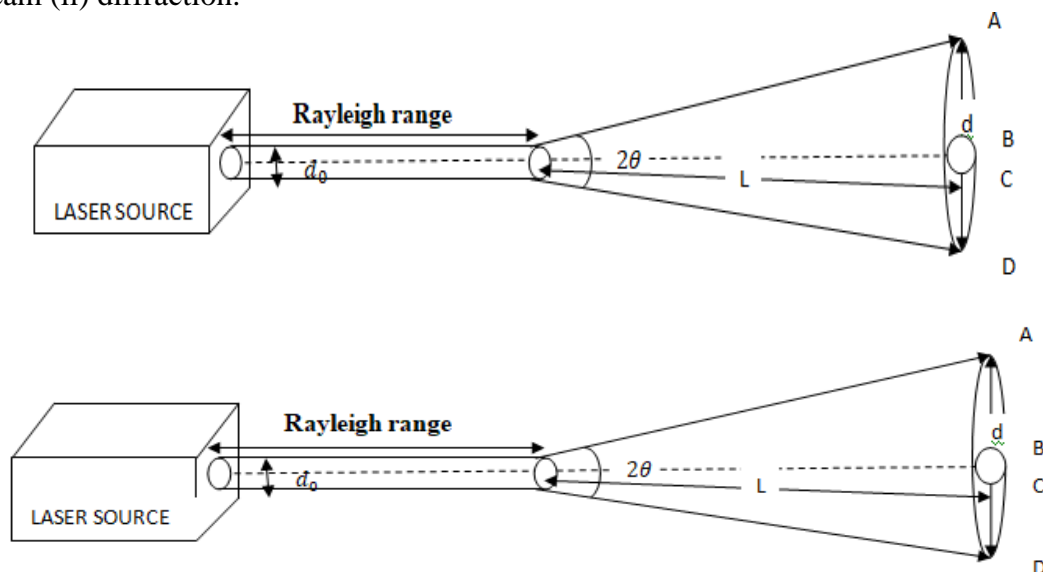
Figure 5 : a- Divergence of a LASER beam
