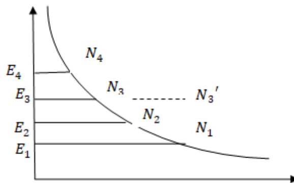
Figure 2: Population inversion
