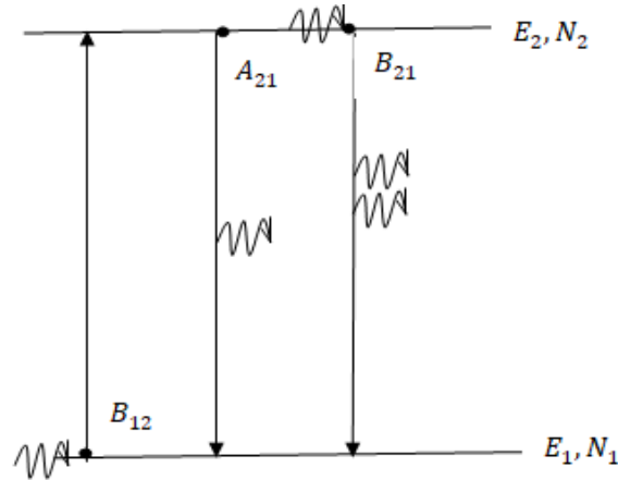
Figure 3: Einstein’s Coefficients
